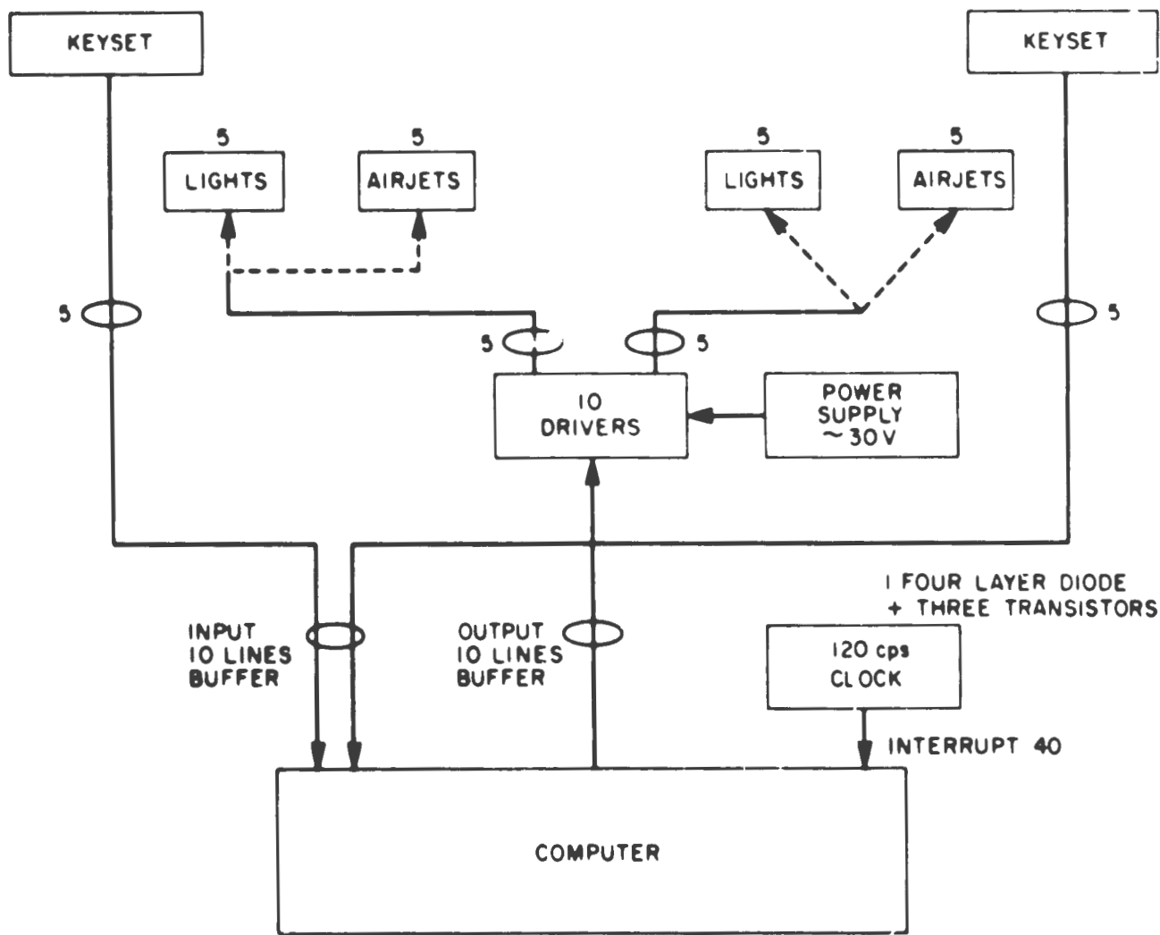
FIG. B-4 BLOCK DIAGRAM OF EQUIPMENT INTERCONNECTION
