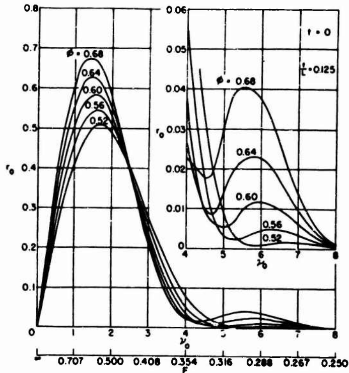
Figure 28 - Wave-Resistance Coefficients r_0 = \frac{R}{4\pi C^2 \rho g b^4/a'} of Symmetrical Bodies Belonging to the Class (2,4,6;\phi;t) = 1 - a_2 \xi^2 - a_4 \xi^4 - a_6 \xi^6 Over \gamma_0 = 1/2F^2 and F = U/\sqrt{gL} t = 0
