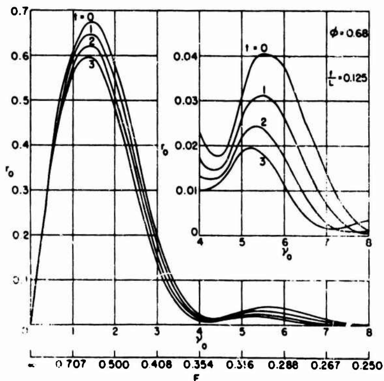
Figure 35 - Wave-Resistance Coefficients r_0 = \frac{R}{4\pi C^2 \rho g b^4/a} , of Symmetrical Bodies Belonging to the Class (2,4,6; \phi ;t) = -a_2 \xi^2 - a_4 \xi^4 - a_6 \xi^6 Over \gamma_0 = 1/2F^2 and F = U/\sqrt{gL} \phi = 0.68
