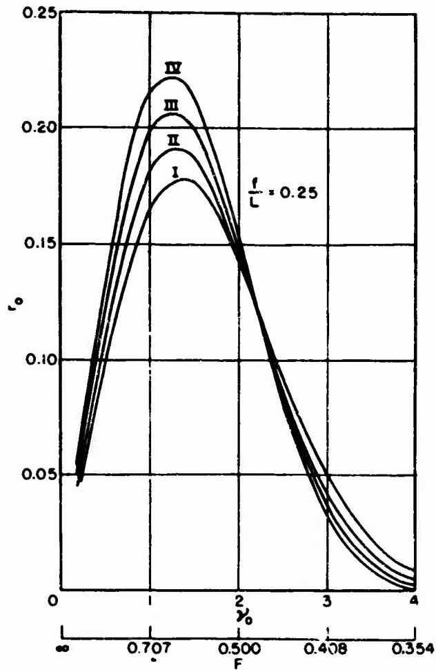
Figure 17 - Total Wave-Resistance Coefficients r_o of the TMB Models Shown in Figures 14 and 15, f/L = 0.25
