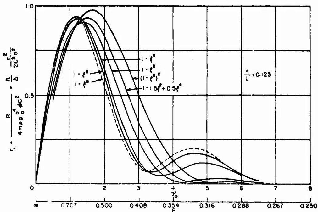
Figure 12 - Wave-Resistance Coefficients r_1 = \frac{r_0}{\phi} = \frac{R}{\Delta} \frac{a^2}{2C^2 b^2} of Symmetrical Bodies Shown on Figure 4, f/L = 0.125
