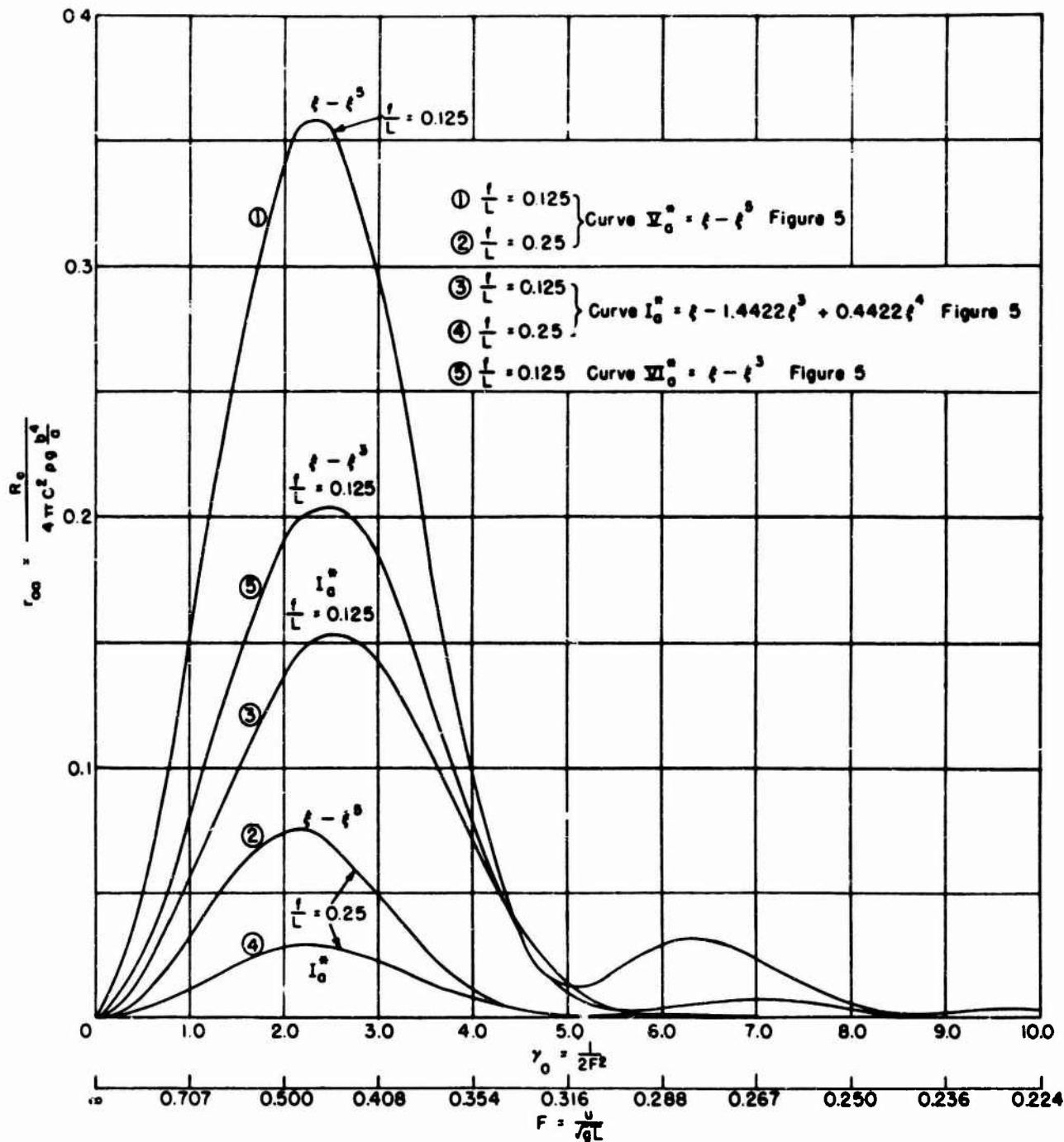
Figure 19 - Wave-Resistance Coefficients r_{oa} Due to Antisymmetrical Distributions Following Figure 5
