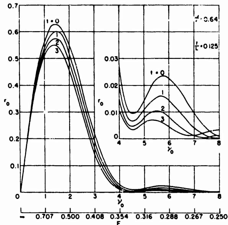
Figure 34 - Wave-Resistance Coefficients r_0 = \frac{R}{4\pi C^2 \rho g b^4/a} , of Symmetrical Bodies Belonging to the Class (2,4,6; \phi ;t) = 1 - a_2 \xi^2 - a_4 \xi^4 - a_6 \xi^6 Over \gamma_0 = 1/2F^2 and F = U/\sqrt{gL} \phi = 0.64
