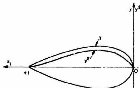
Figure 3a - Landweber's Axes
