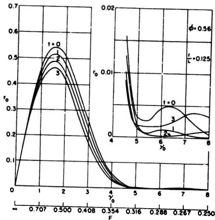
Figure 32 - Wave-Resistance Coefficients r_0 = \frac{R}{4\pi C^3 \rho g b^4/a} , of Symmetrical Bodies Belonging to the Class (2,4,6; \phi ;t) = 1 - a_2 \xi^2 - a_4 \xi^4 - a_6 \xi^6 Over \gamma_0 = 1/2F^2 and F = U/\sqrt{gL} \phi = 0.56
