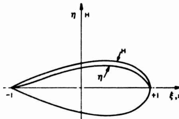
Figure 3b - Present Axes
