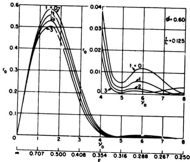
Figure 33 - Wave-Resistance Coefficients r_0 = \frac{R}{4\pi C^3 \rho g b^4/a} , of Symmetrical Bodies Belonging to the Class (2,4,6; \phi ;t) = 1 - a_2 \xi^2 - a_4 \xi^4 - a_6 \xi^6 Over \gamma_0 = 1/2F^2 and F = U/\sqrt{gL} \phi = 0.60
