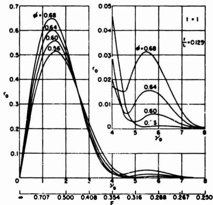
Figure 29 - Wave-Resistance Coefficients r_0 = \frac{R}{4\pi C^2 \rho g b^4/a'} of Symmetrical Bodies Belonging to the Class (2,4,6;\phi;t) = 1 - a_2 \xi^2 - a_4 \xi^4 - a_6 \xi^6 Over \gamma_0 = 1/2F^2 and F = U/\sqrt{gL} t = 1
