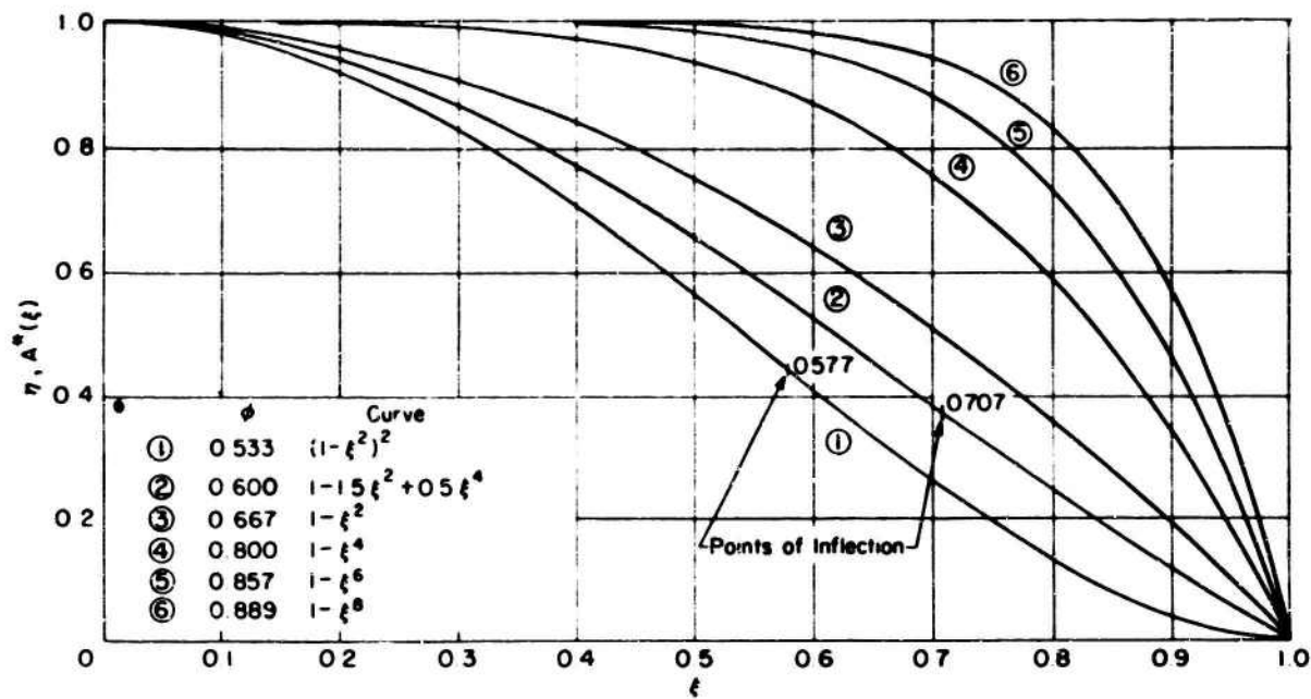
Figure 4 - Dimensionless Sectional-Area Curves A^*(\xi) (Doublet Distributions \mu^*(\xi) ) of Some Simple Bodies Symmetric with Respect to the Midship Section
