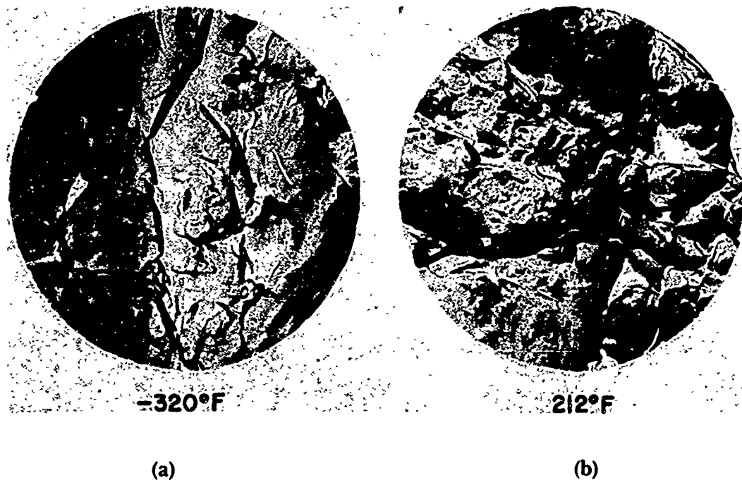
Fig. 8 — Electron microscope fractographs of a low interstitial Ti-6Al-4V alloy fracture surface showing a dimpled rupture. Fracture surface generated at (a) -320°F and (b) +212°F, original magnification 4000X; printing reduction 58-1/2%.
