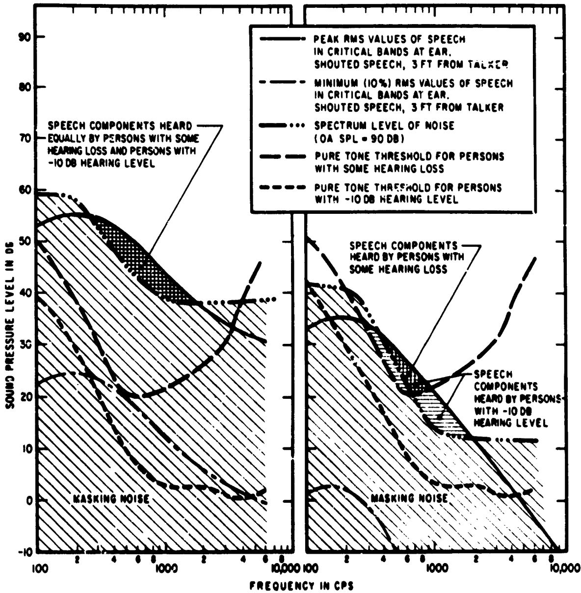
Fig. 11b. THE EFFECT OF WEARING EARPLUGS IN MODERATE NOISE FOR PERSONS WITH NORMAL HEARING AND PERSONS WITH SOME HEARING LOSS
