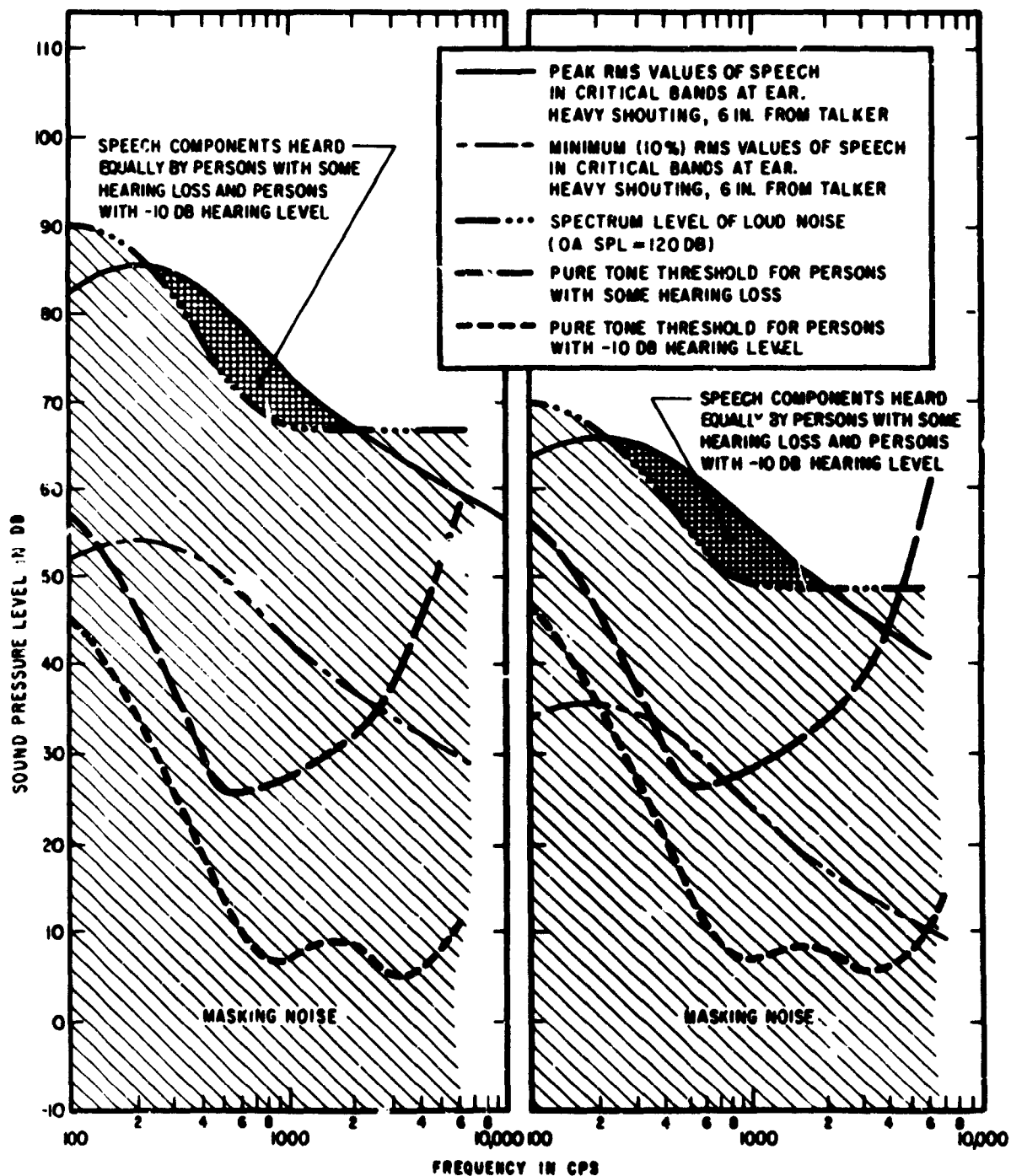
Fig. 11c. THE EFFECT OF WEARING EARPLUGS IN INTENSE NOISE FOR PERSONS WITH NORMAL HEARING AND PERSONS WITH SOME HEARING LOSS
