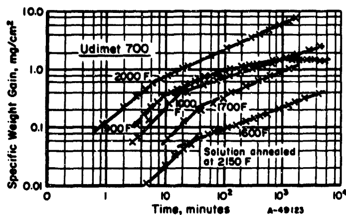
FIGURE 13. LOGARITHMIC PLOT OF SPECIFIC WEIGHT GAIN AGAINST TIME FOR A SINGLE HEAT OF CAST UDIMET 700 (16)
