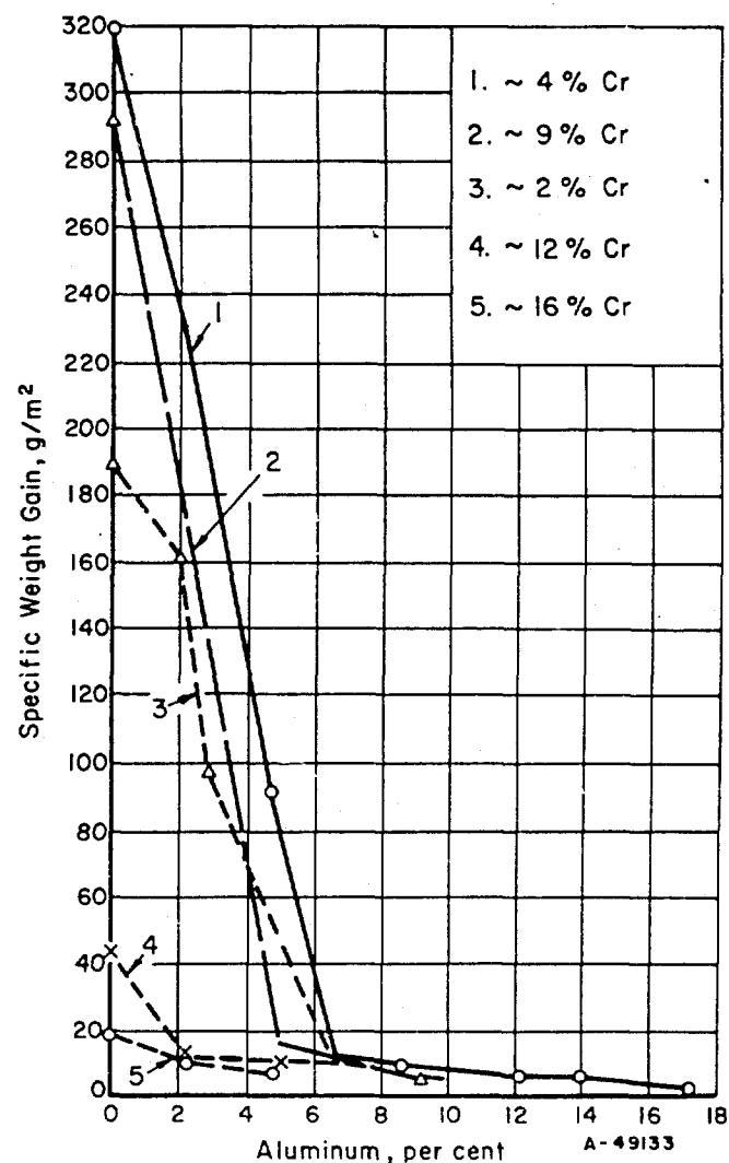
FIGURE 6. OXIDATION RESISTANCE OF ALLOYS CONTAINING VARIOUS AMOUNTS OF CHROMIUM AND ALUMINUM (1)
