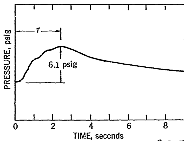
Figure 1 Typical Pressure History Record Obtained During Combustion of 50 Volume Percent \text{CF}_2\text{Br}_2 in an Oxygen Atmosphere in a 2-foot Diameter Sphere
