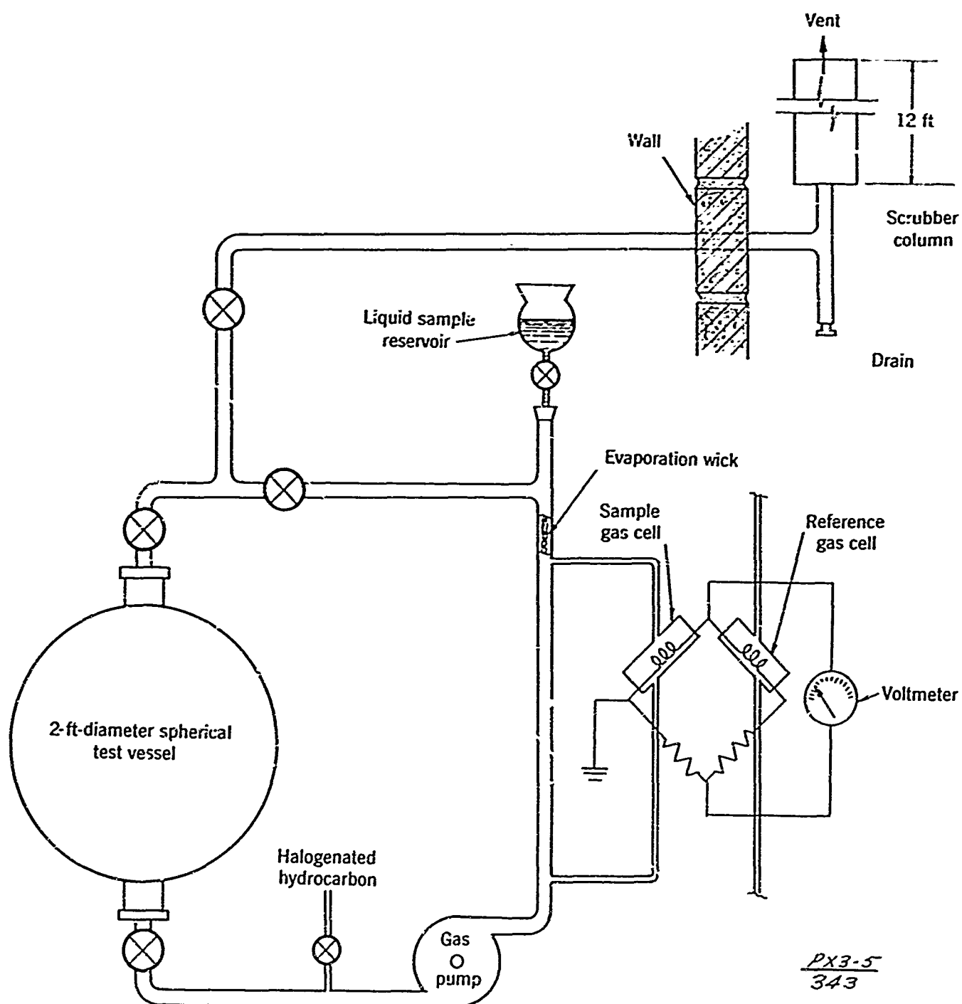
Figure 2 Apparatus Used to Measure Maximum Explosion Pressures During Combustion of Confined Gas Mixtures
