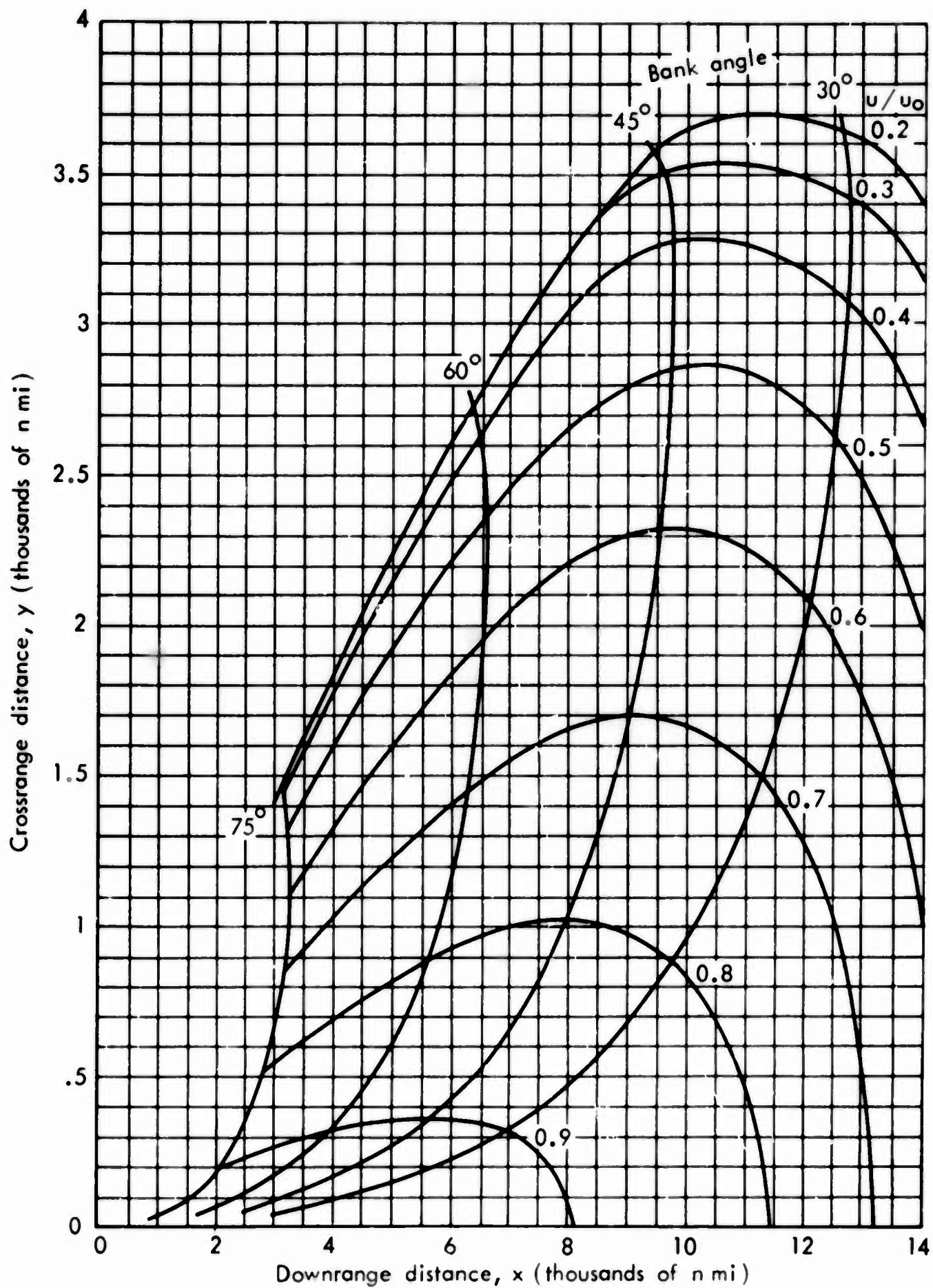
Fig.8—Ground trace during turn, L/D = 3
