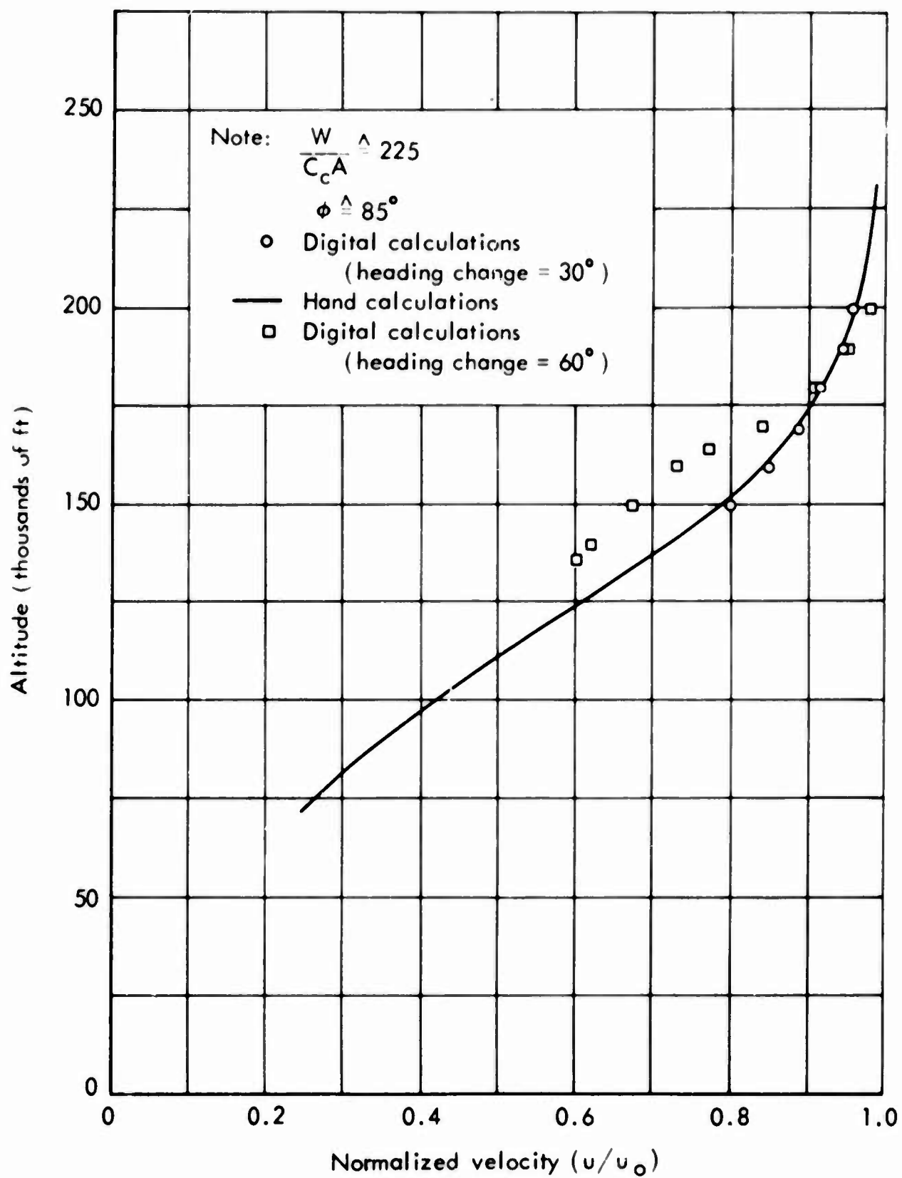
Fig. 18— Comparison of altitude - velocity profiles, \phi = 85^\circ
