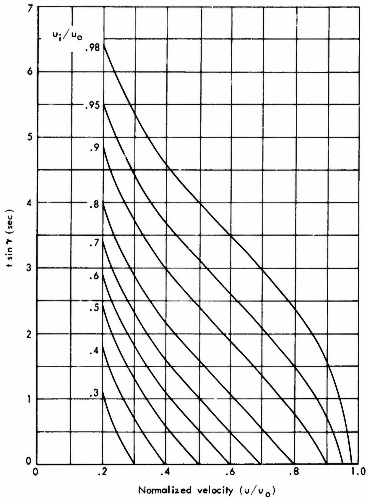
Fig. 11—Time of flight ( \phi = 90^\circ )
