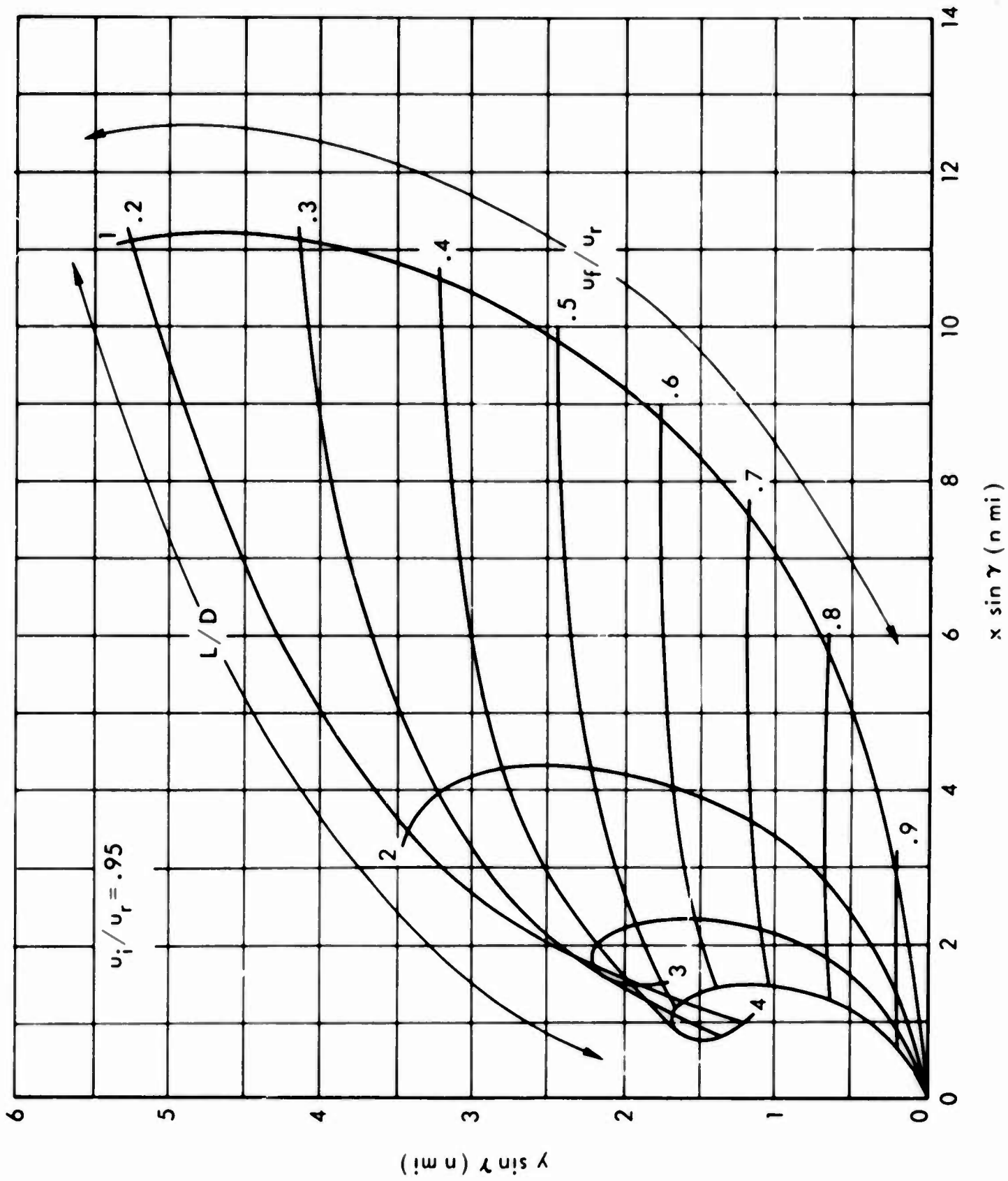
Fig. 14—Ground trace for \phi = 90^\circ ( u_i = 0.95 u_r )
