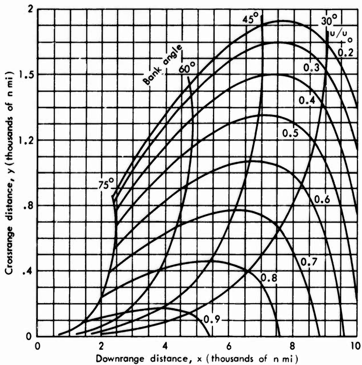
Fig.7—Ground trace during turn, L/D = 2
