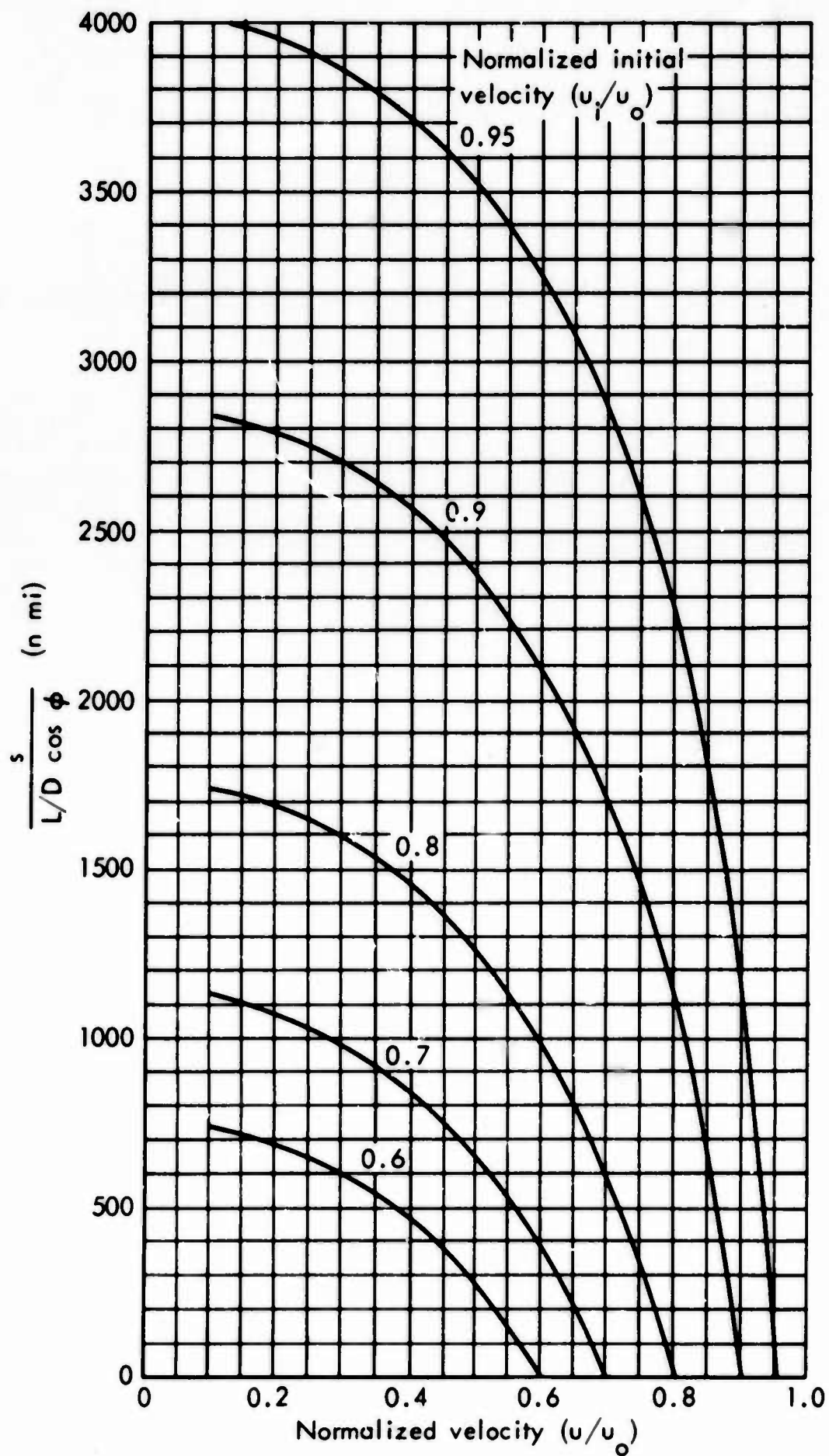
Fig.5—Flight path length
