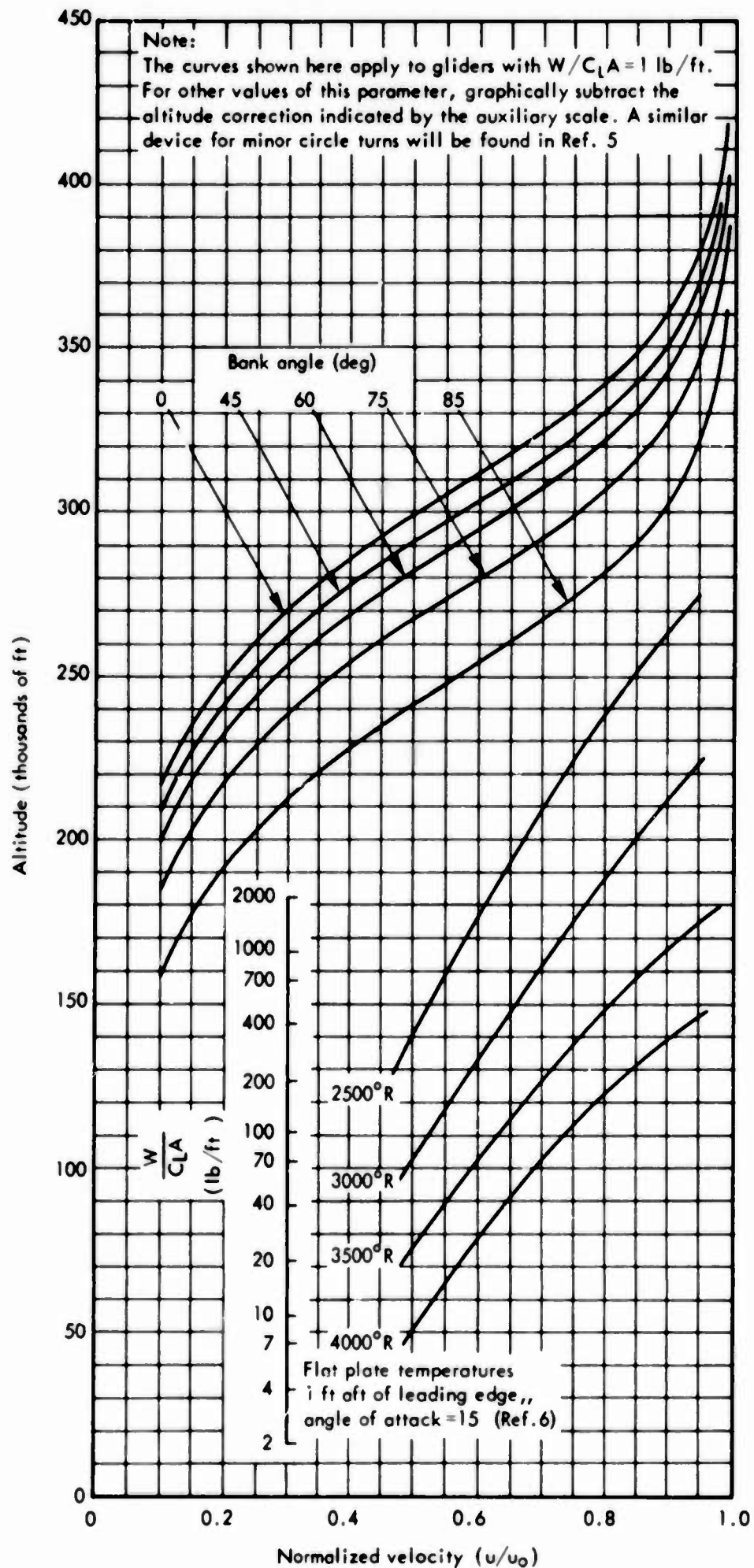
Fig. 3—Glide reentry trajectories for constant bank angle control
