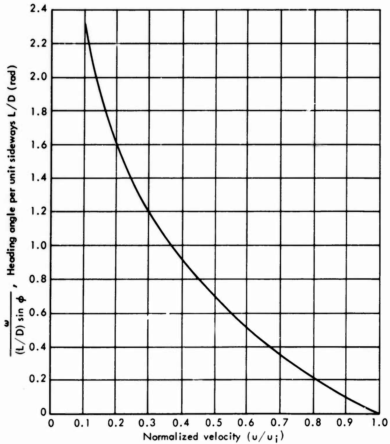
Fig.2—Heading angle-velocity relation
