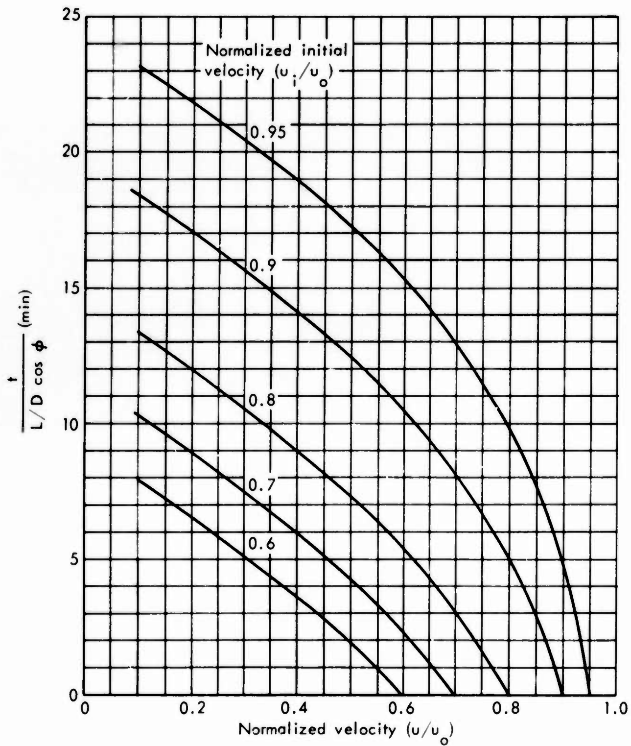
Fig.4—Time of flight
