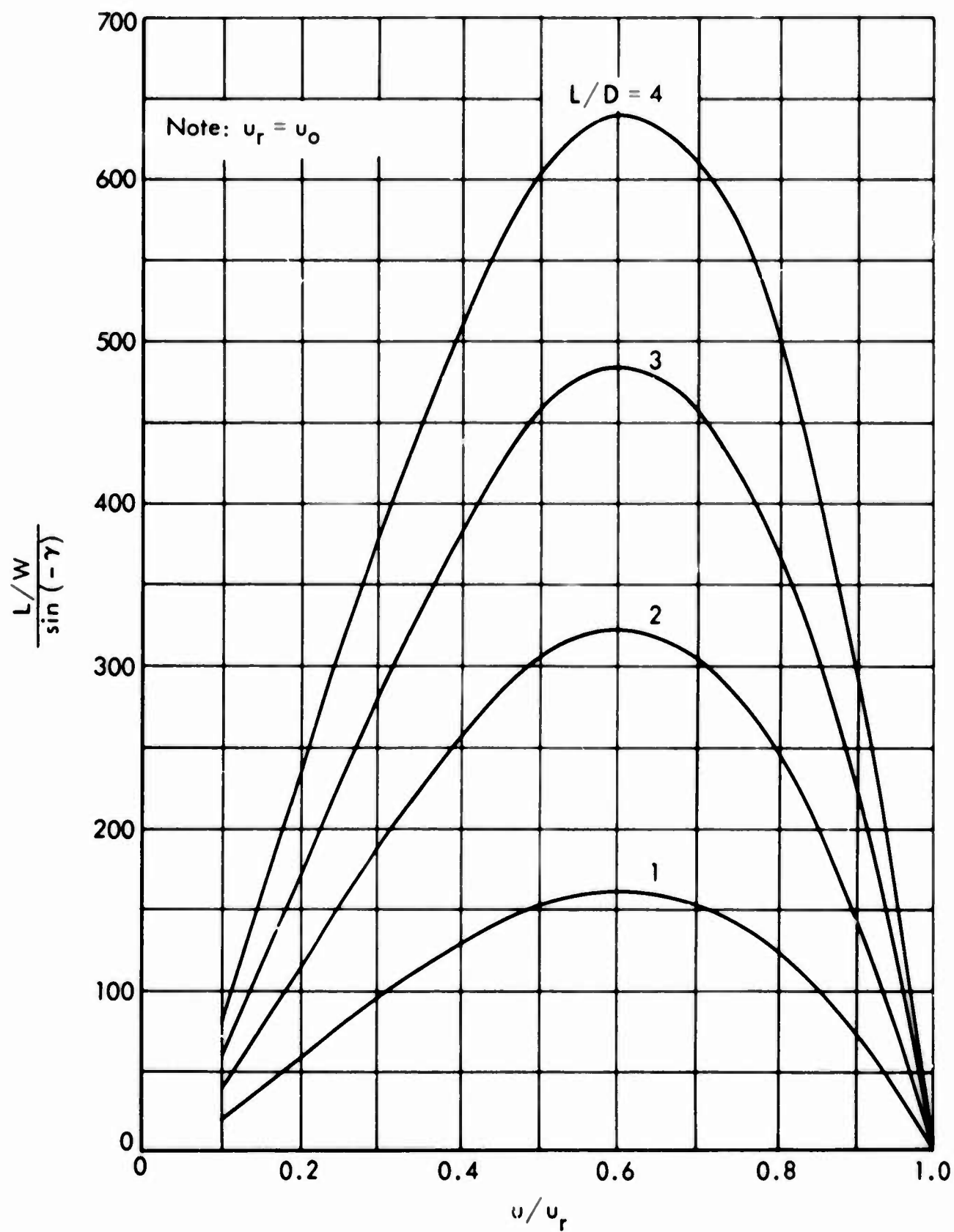
Fig. 12—Normal load factor for \phi = 90^\circ
