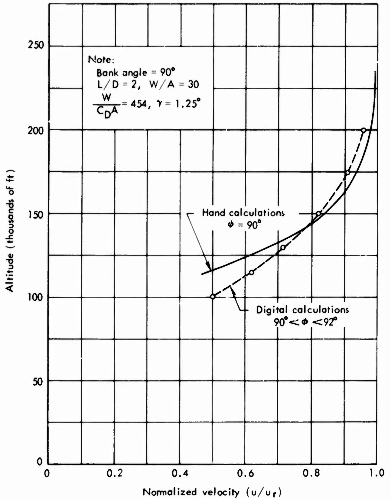
Fig. 17— Comparison of velocity - altitude profiles, \phi = 90^\circ
