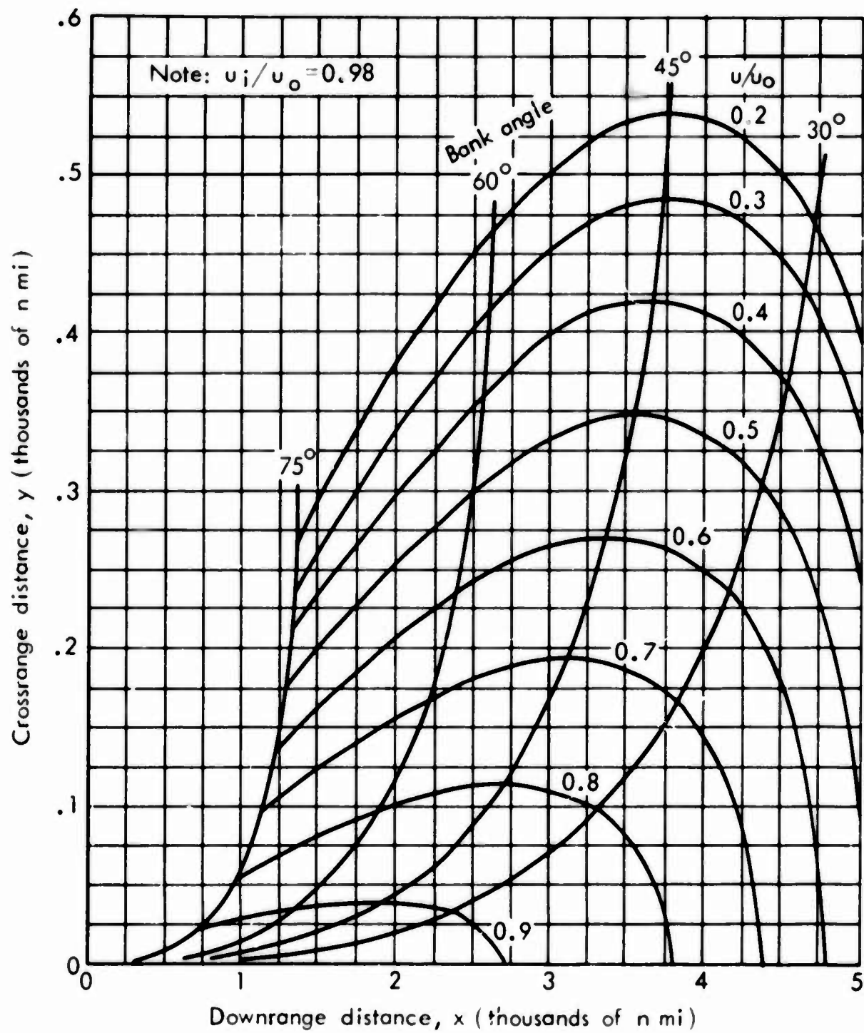
Fig. 6—Ground trace during turn, L/D = 1
