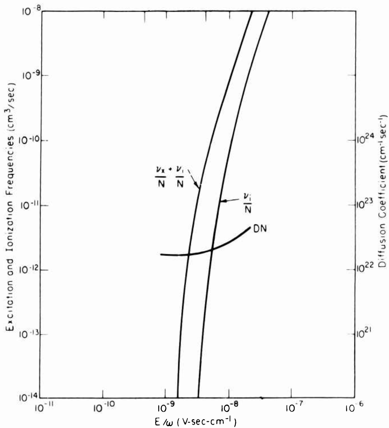
Figure IV - 7 Electronic Excitation and Ionization in N_2 for \omega \gg \nu_m
