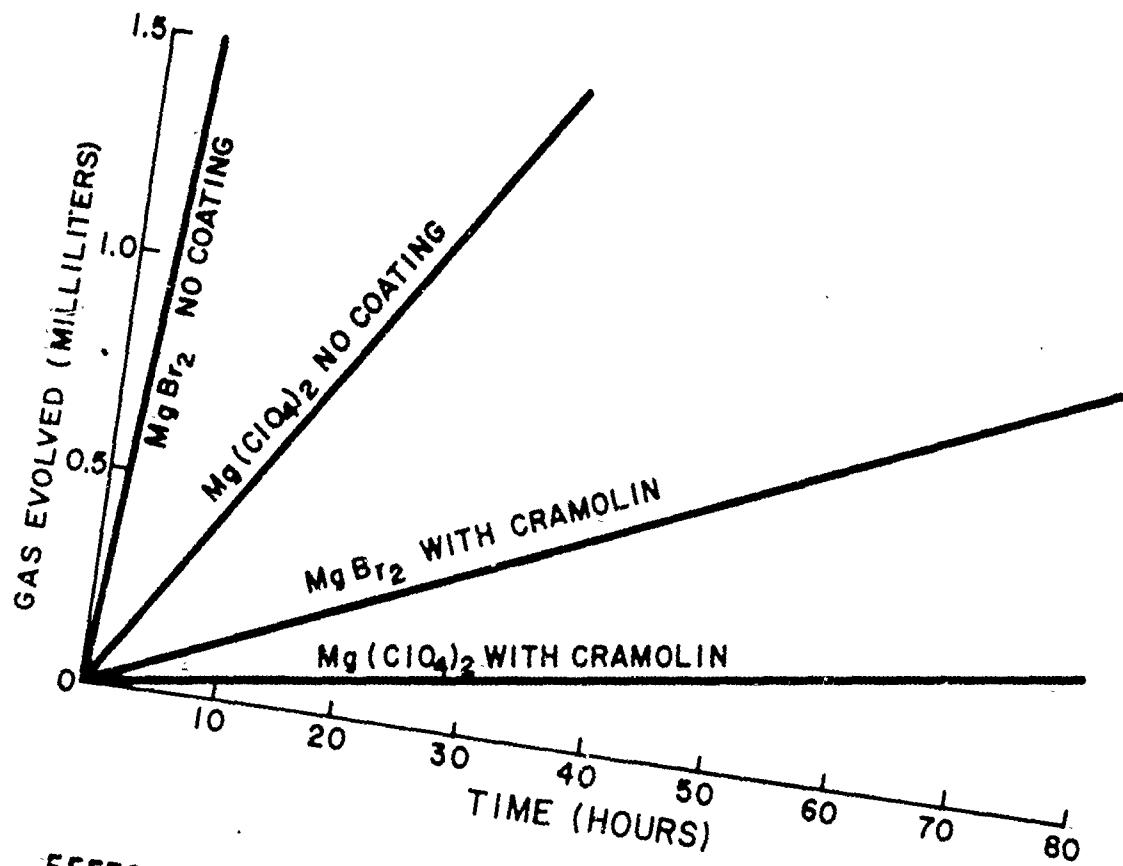
EFFECT OF DILUTE CRAMOLIN ON THE GAS EVOLUTION FOR AZ-21 MAGNESIUM IN \text{MgBr}_2 & \text{Mg}(\text{ClO}_4)_2 ELECTROLYTES
