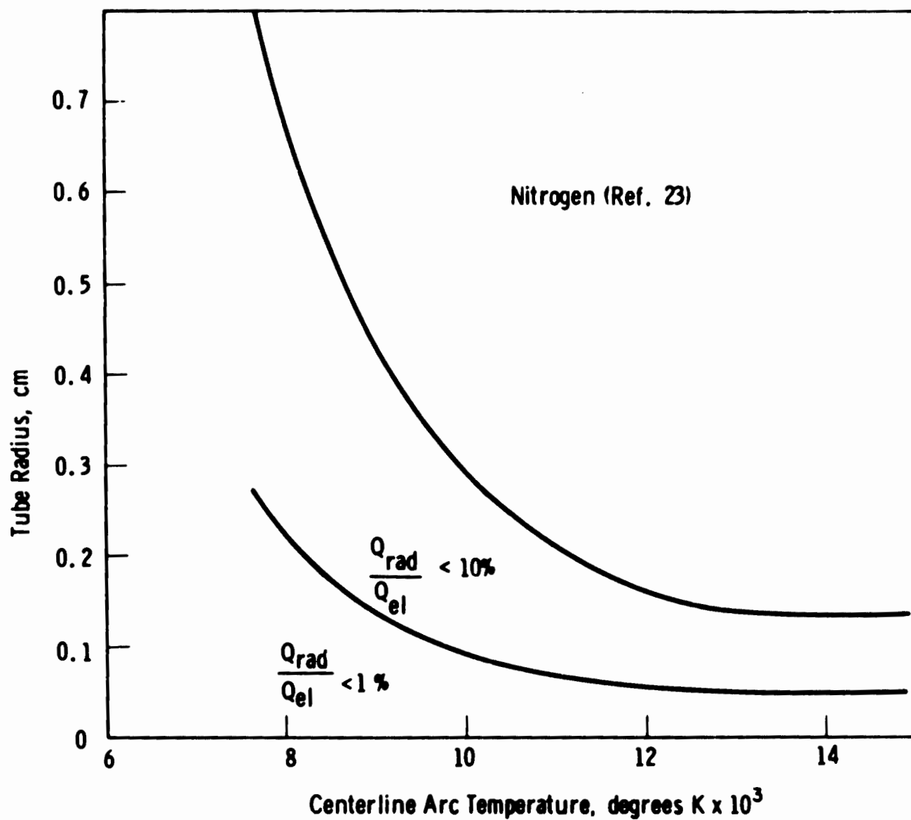
Figure 2. Map Showing Regions in the Tube Radius—Arc Temperature Plane Where Radiation is Negligible
