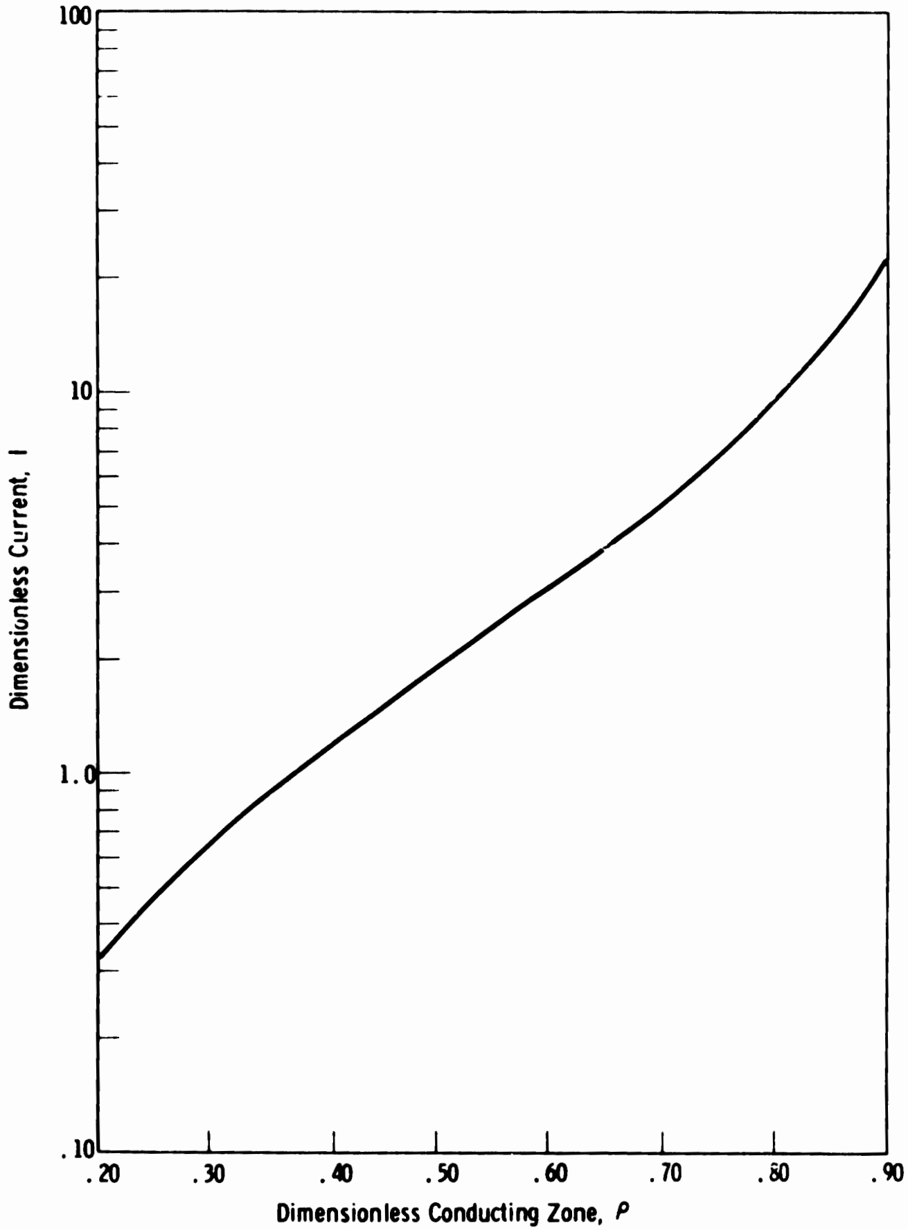
Figure 15. Dimensionless Current vs. Conducting Zone Radius for the DC Arc
