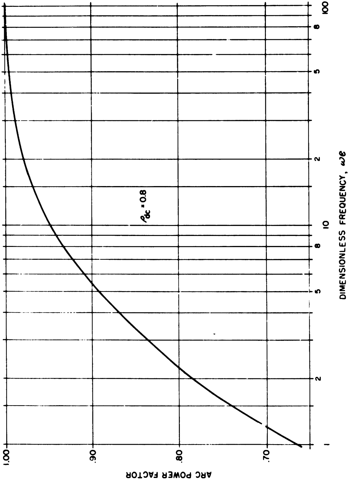
Figure 27. Theoretical Power Factor vs. \omega\epsilon for an Isolated AC Arc
