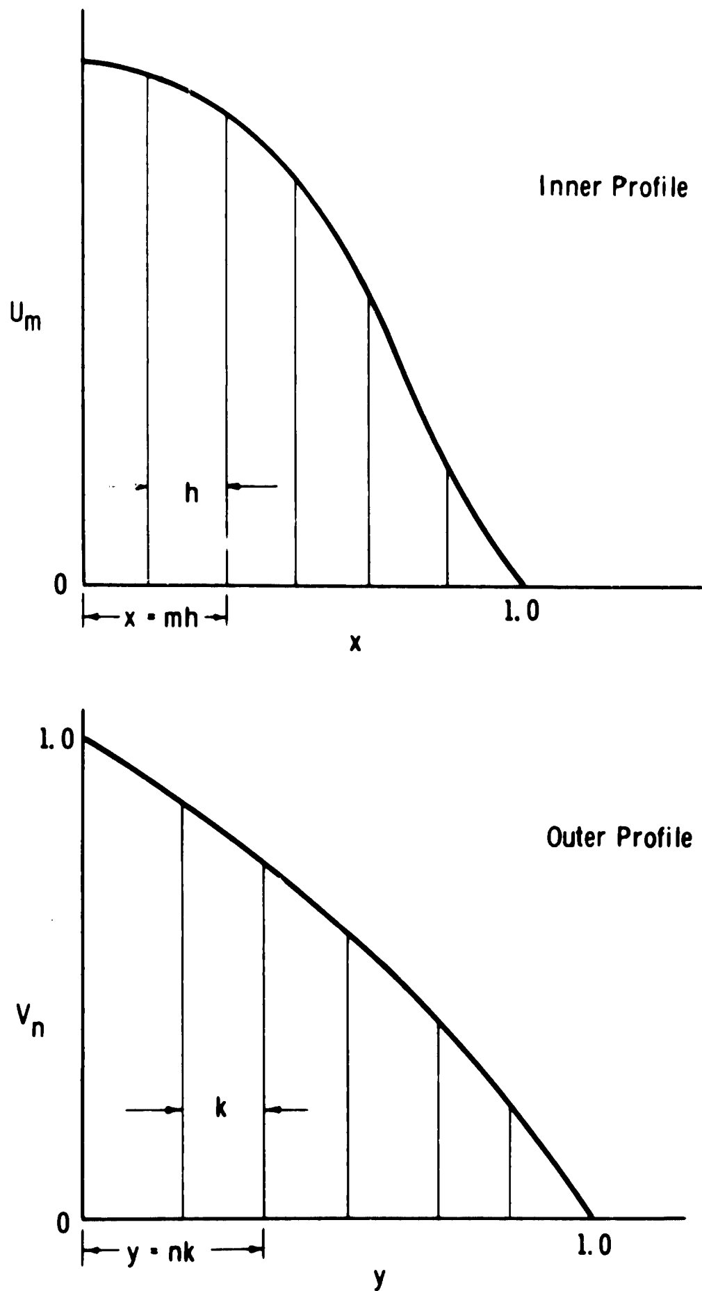
Figure 14. Coordinate System for the Finite-Difference Scheme
