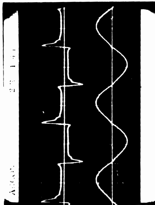
Figure 36. Experimental Voltage and Current Waveforms for an Argon Arc in a 1/4 in. Tube
