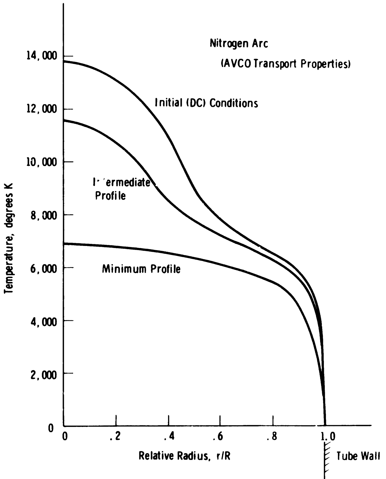
Figure 29. Theoretical Temperature Profiles for a Nitrogen AC Arc
