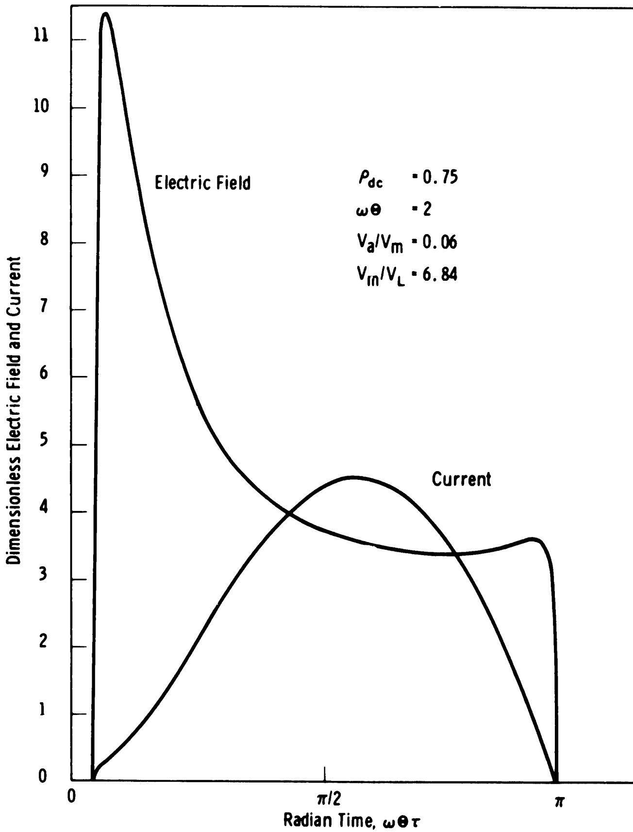
Figure 42. Theoretical Waveforms of Electric Field Strength and Dimensionless Current Including the Effects of an External Circuit
