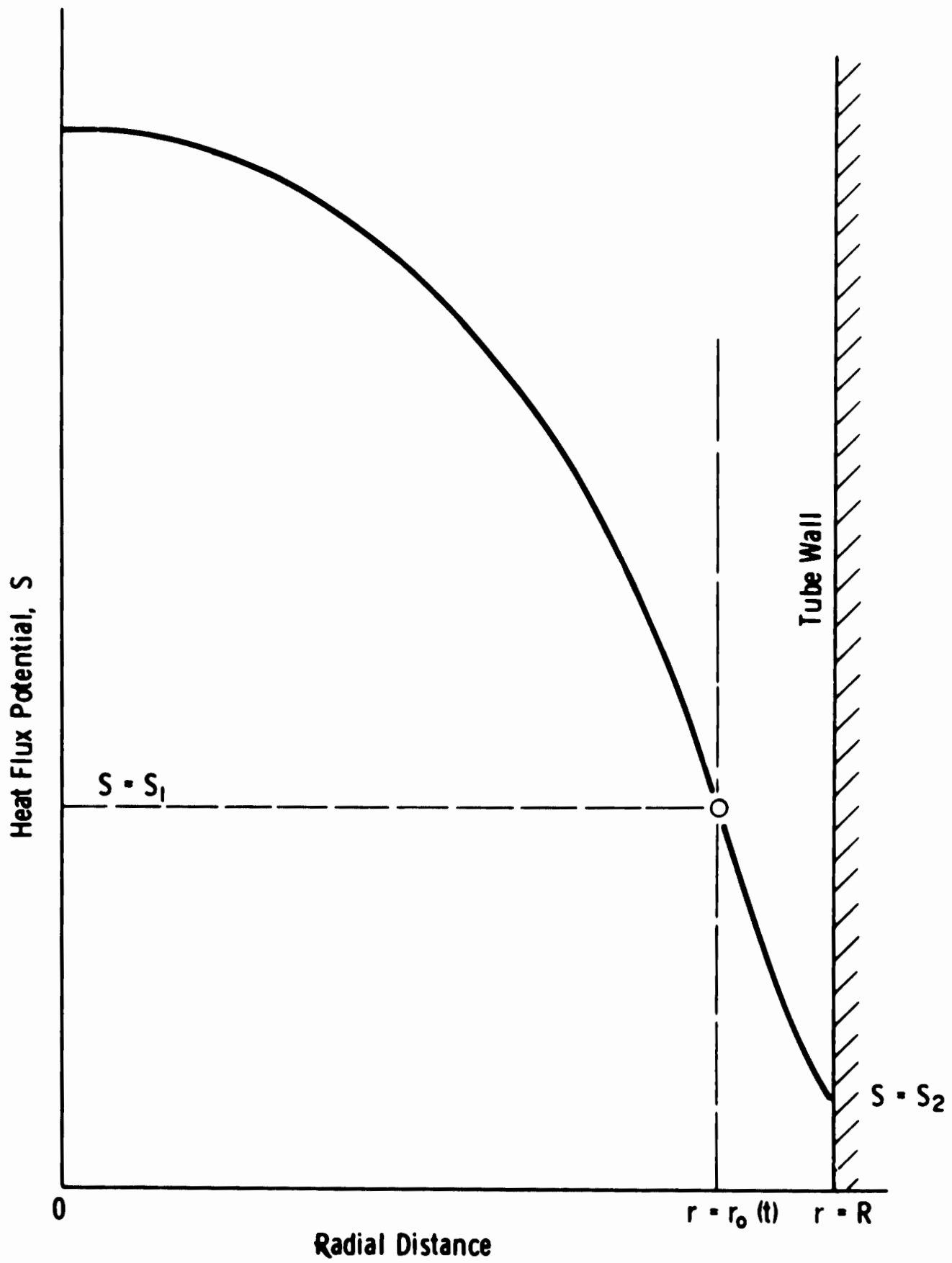
Figure 6. Coordinate System for the Cylindrically Symmetric Arc
