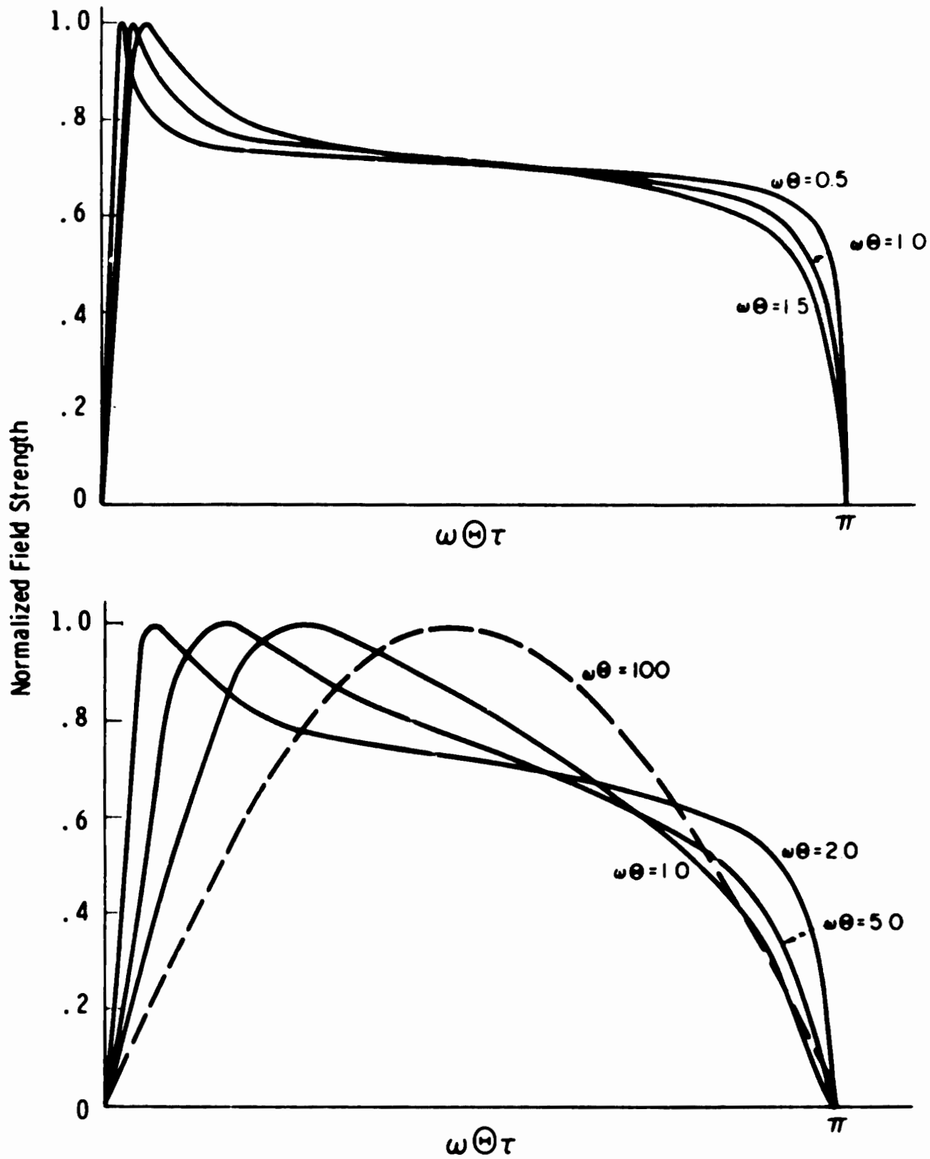
Figure 10. Electric Field Waveforms for a Constant Radius AC Arc
