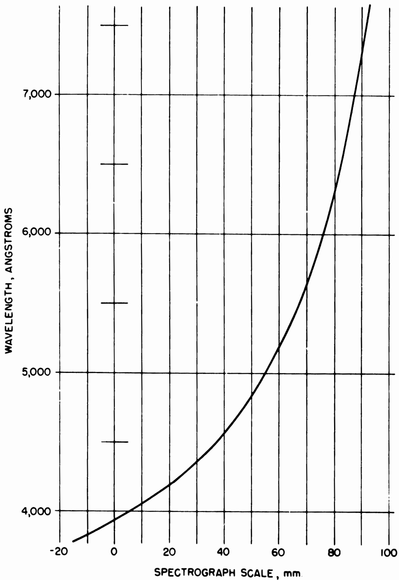
Figure 32b. Wavelength Conversion Scale for Spectra of Figure 32a
