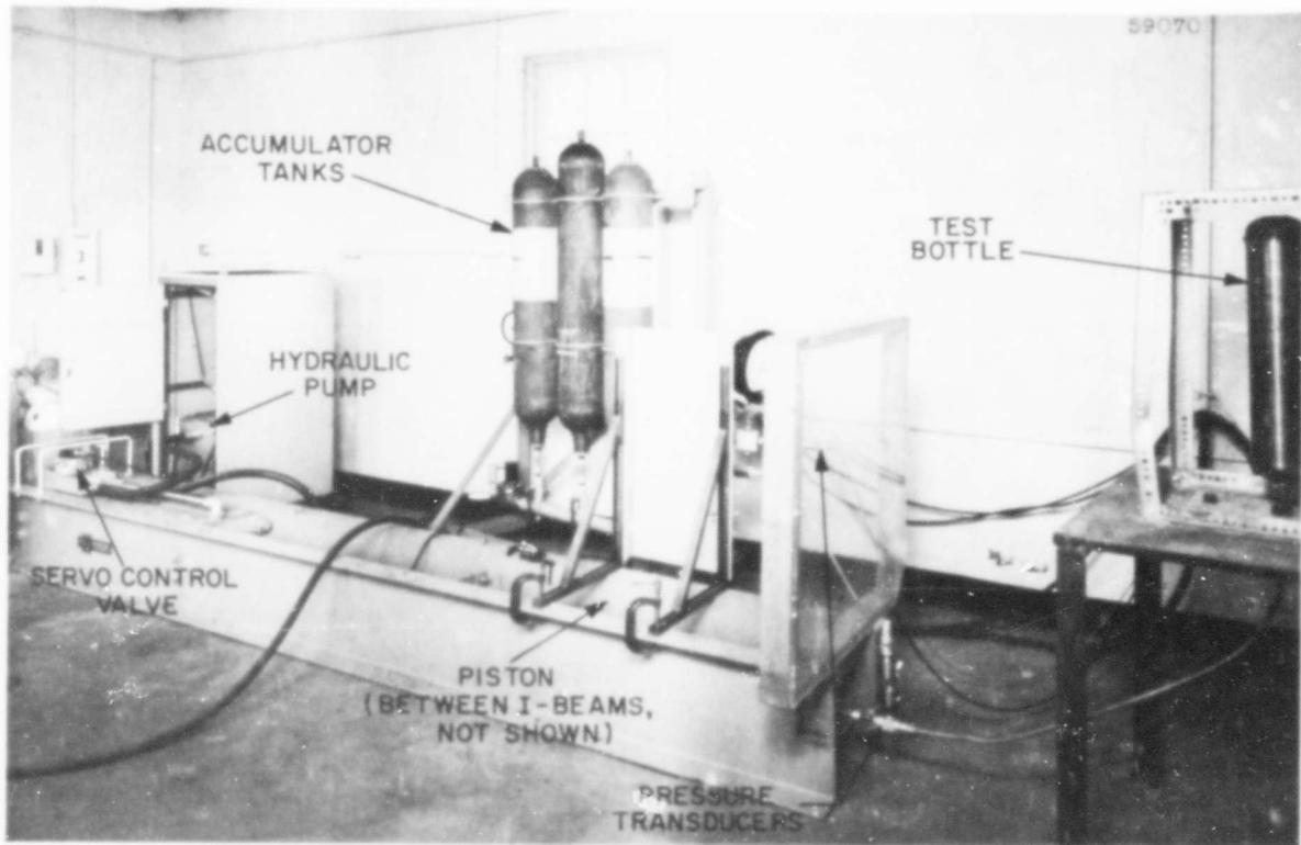
Fig. 3 - Bottle-test assembly
