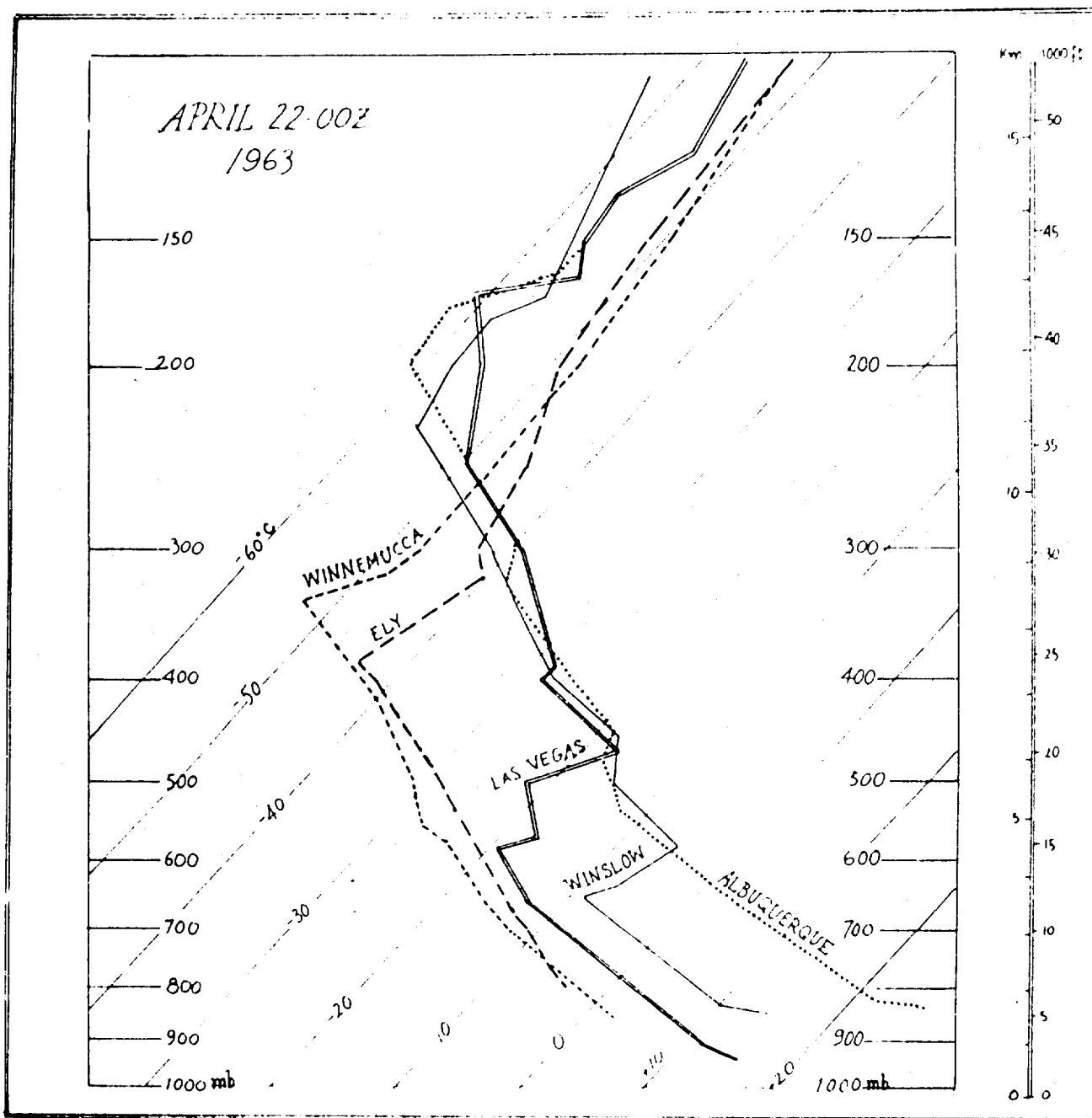
Temperature versus Pressure for Radiosonde Stations, April 22, Cross Section Figure 17
