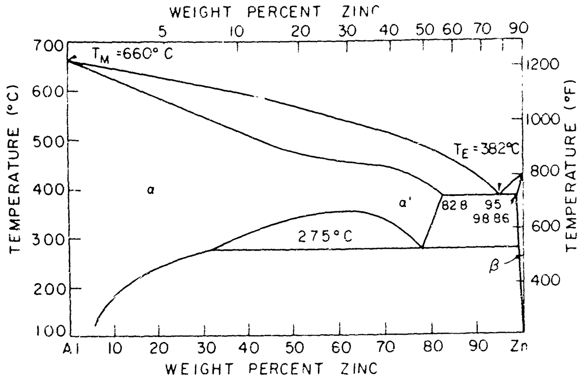
Fig. 3: Aluminum-zinc equilibrium phase diagram (A S M , Metals Handbook , 1948)
