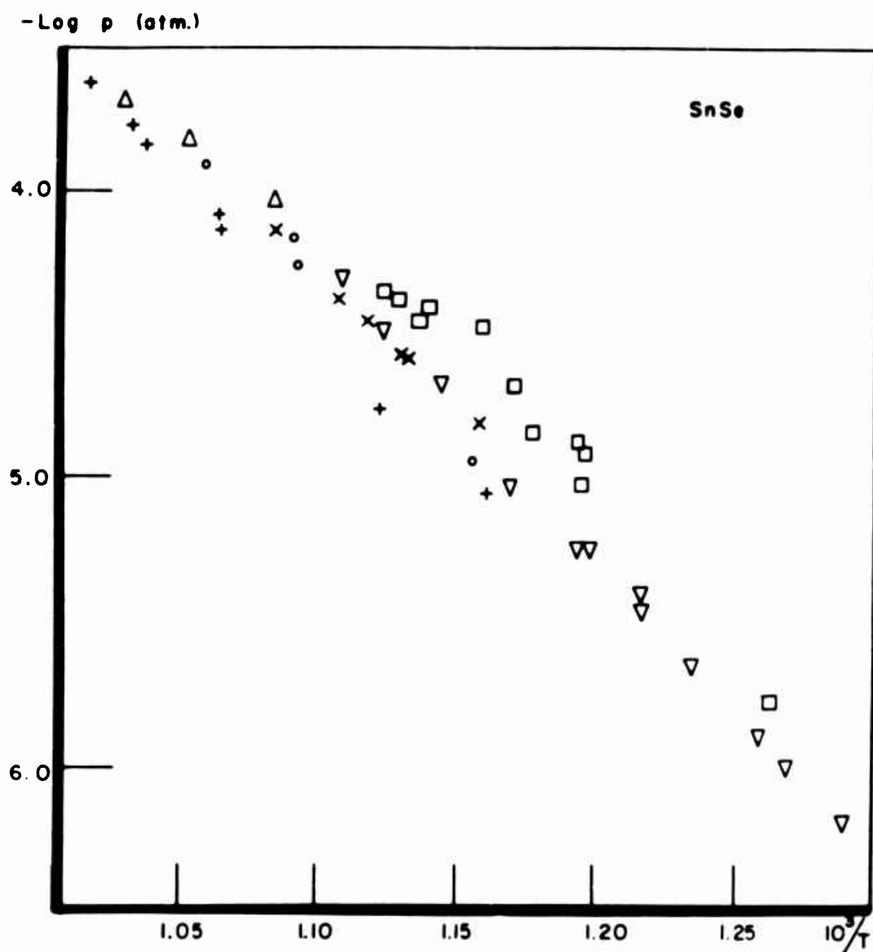
Fig. 1. Vapor pressure of SnSe
