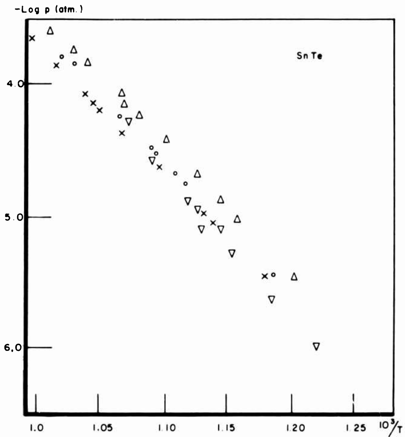
Fig. 2. Vapor Pressure of SnTe
