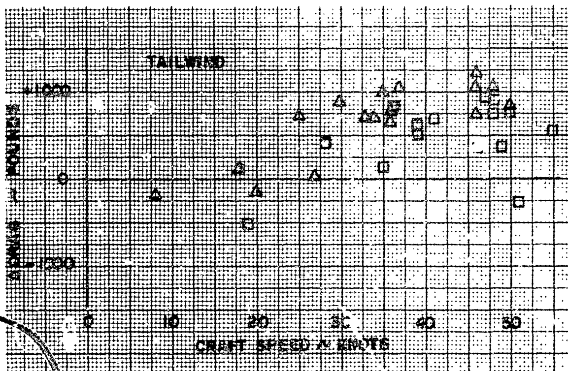
Figure 6-22. Deviation of Test Data from Theory, Sea State 0, Tailwind, Drag vs Craft Speed
