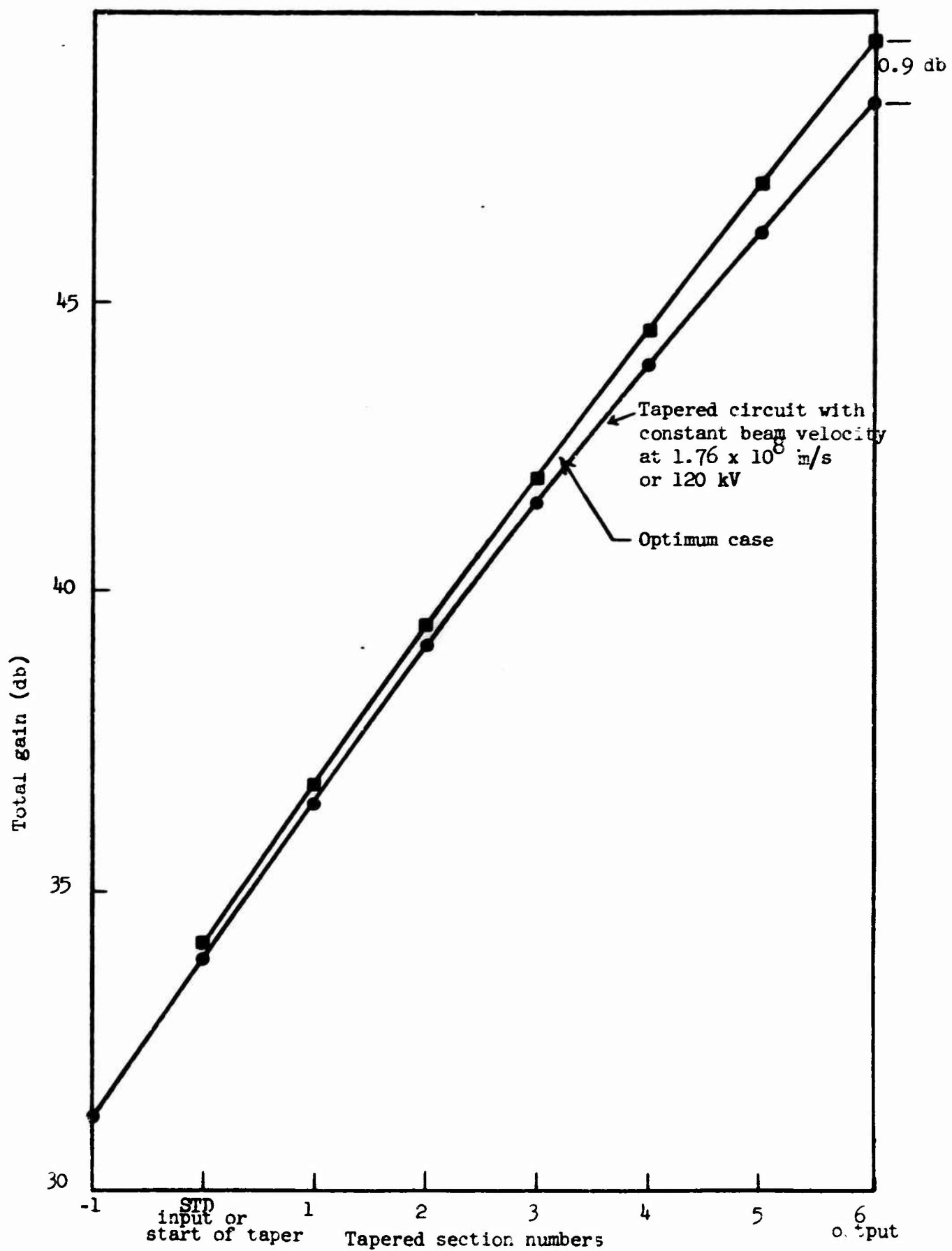
FIG. 2.22--Total gain vs tapered section number at 120 kV for f = 2092 Mc/s.
