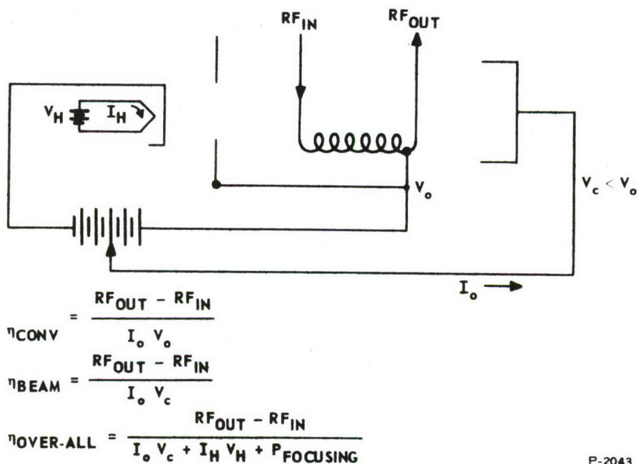
Figure 4-2 - Schematic Diagram of a TWA Defining the Various Efficiencies of Interest in Microwave Tubes
