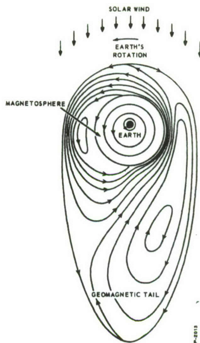
Figure A-3 - Trapped Radiation and the Magnetosphere Showing Probable Distortion Due to the Solar Wind - Polar View
