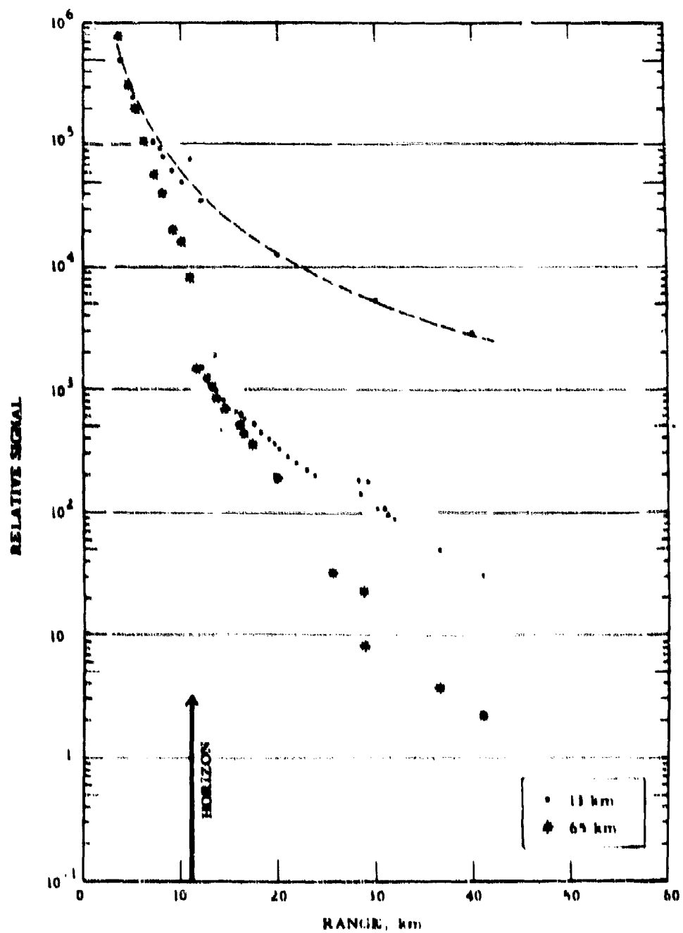
Fig. 1b - Behavior of scattered light as a function of distance for visible radiation (4700A to 7000A) when the meteorological range was 13 and 65 km
