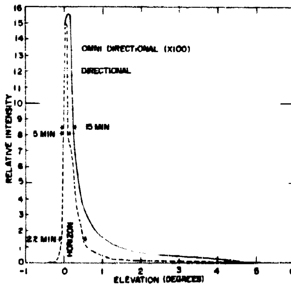
Fig. 9 - Vertical cross section through the region of maximum horizon radiance for directional and omnidirectional light sources below the horizon and 45 km away
