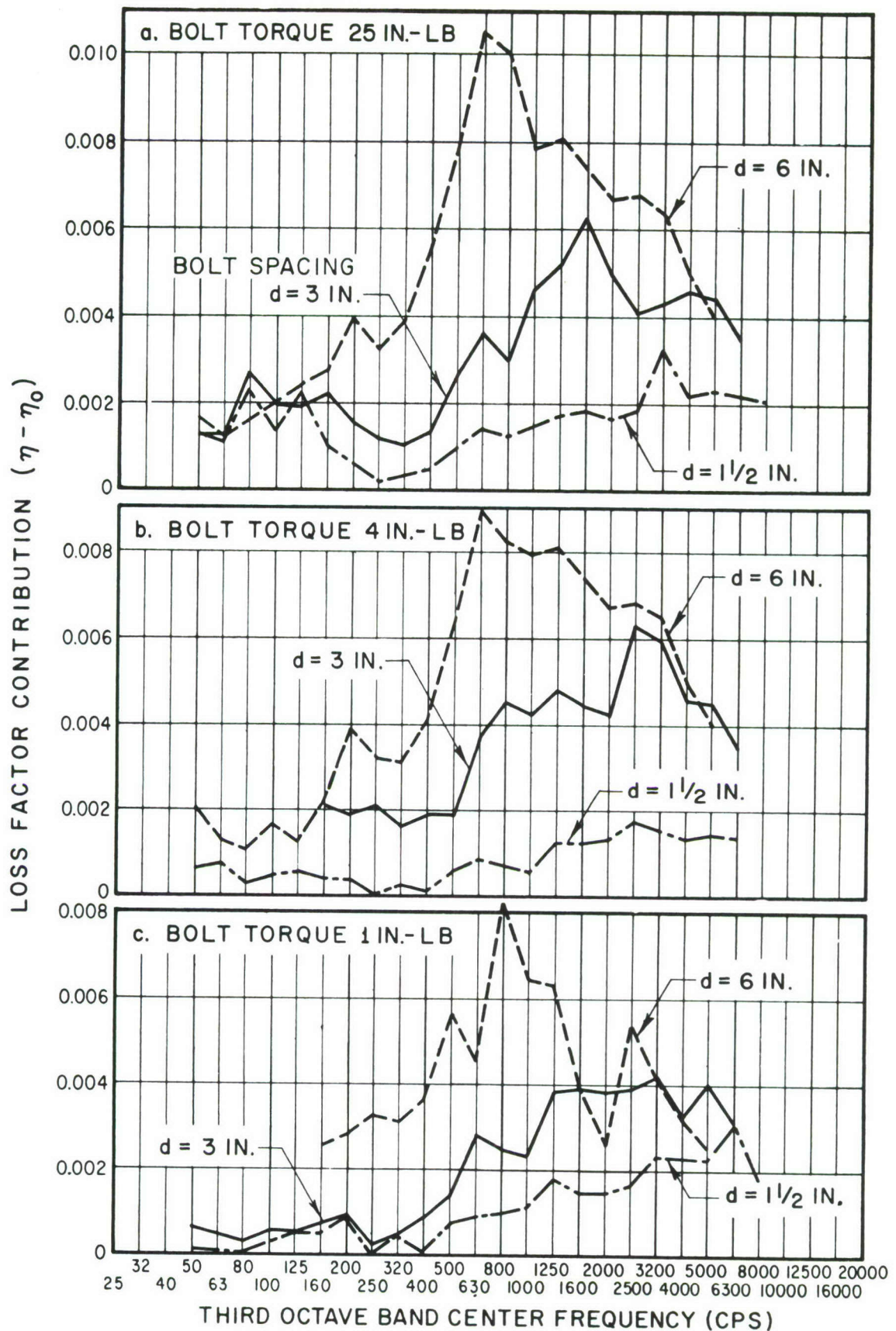
FIG.5 EFFECT OF BOLT SPACING ON LOSS FACTOR CONTRIBUTION BY BEAMS. (1/16 ALUMINUM PLATE AS IN FIG. I, ALL BEAMS ATTACHED)
