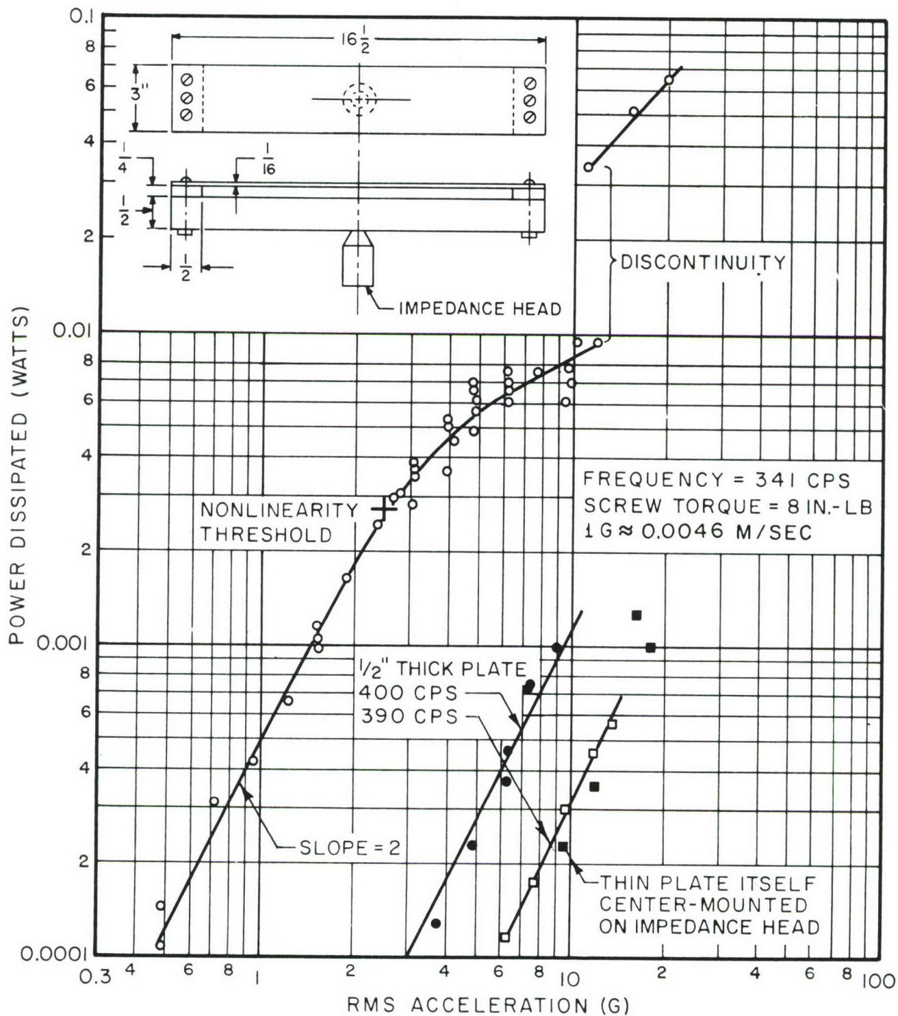
FIG. 32 POWER DISSIPATION AS A FUNCTION OF AMPLITUDE FOR 3rd MODE OF PANEL DRIVEN AT EDGES VIA THICK PLATE
