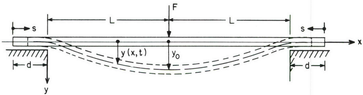
a. GENERAL ARRANGEMENT
