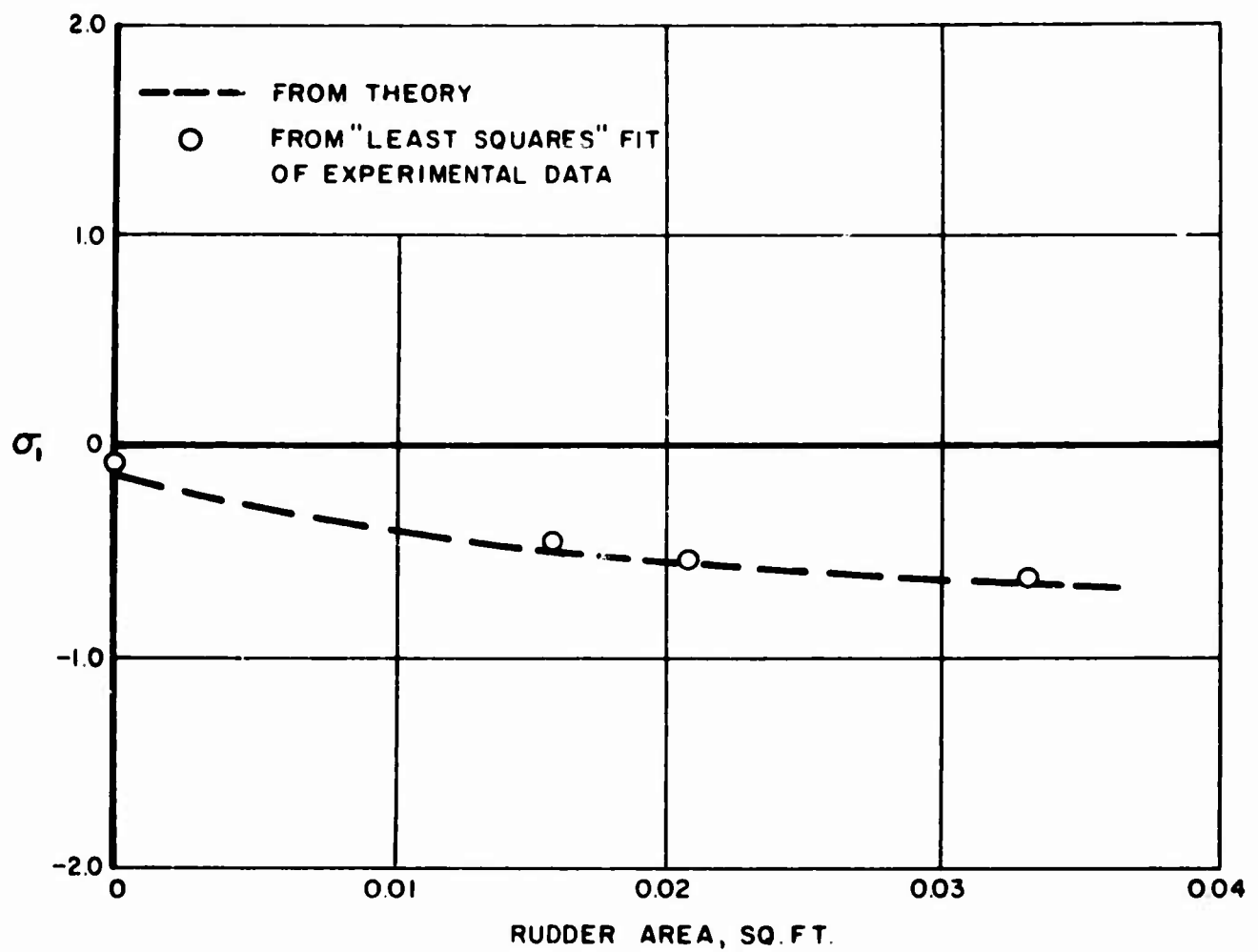
FIGURE B-6. STABILITY INDEX \sigma_1 FOR MODEL 2, SERIES 60, WITH RUDDERS OF VARYING CHORD
