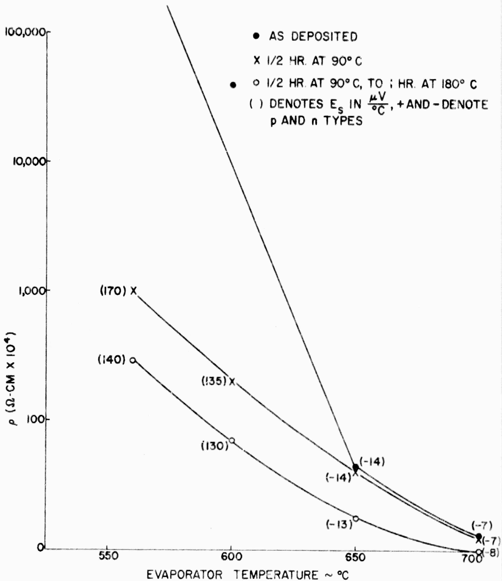
FIG. 3. RESISTIVITY OF Bi-Sb-Te FILMS DEPOSITED ON 23^{\circ}\text{C} GLASS.
