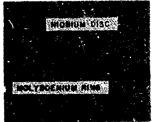
Before (250X) After 2 CNM brazed approx. 1300°C, 2 min., .0005-inch nickel shim
