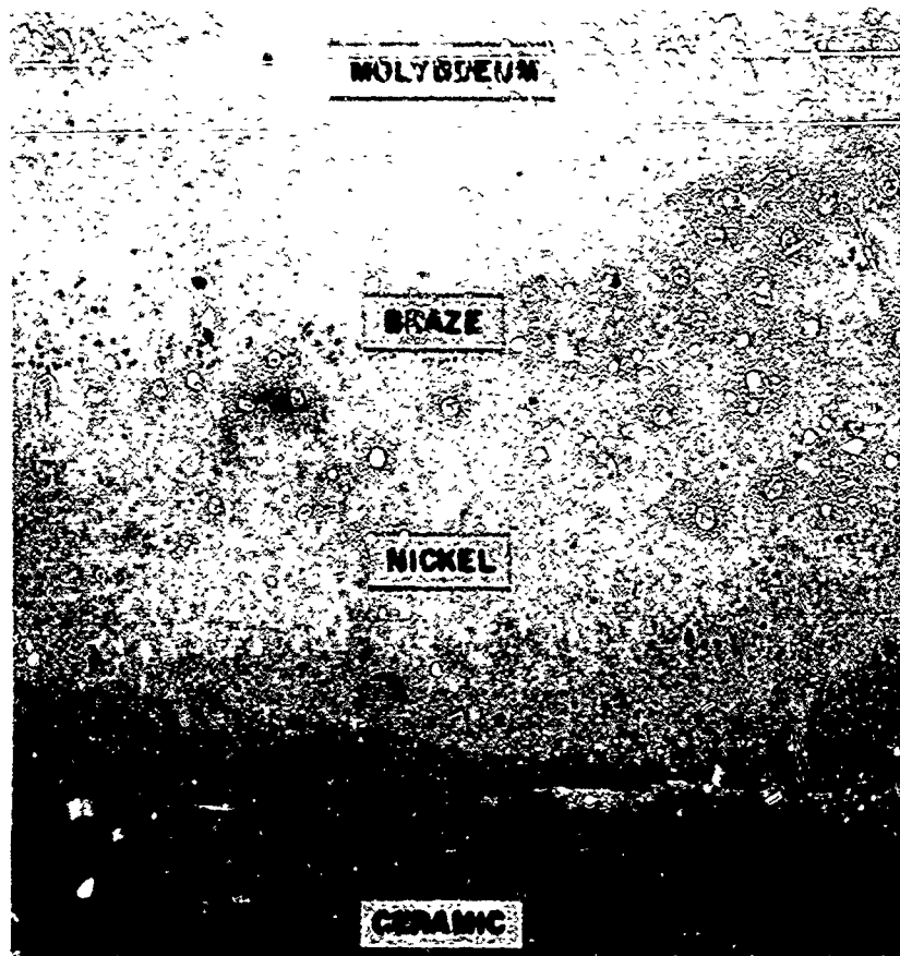
Alumina-to-Molybdenum Seal with Nickel Buffer Washers After 20 Thermal Cycles to 900°C (500X)
