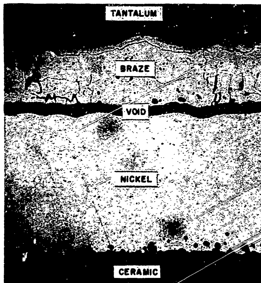
Alumina-to-Tantalum Seal with Nickel Buffer Washers After 240 Hours at 1075°C (500X)
