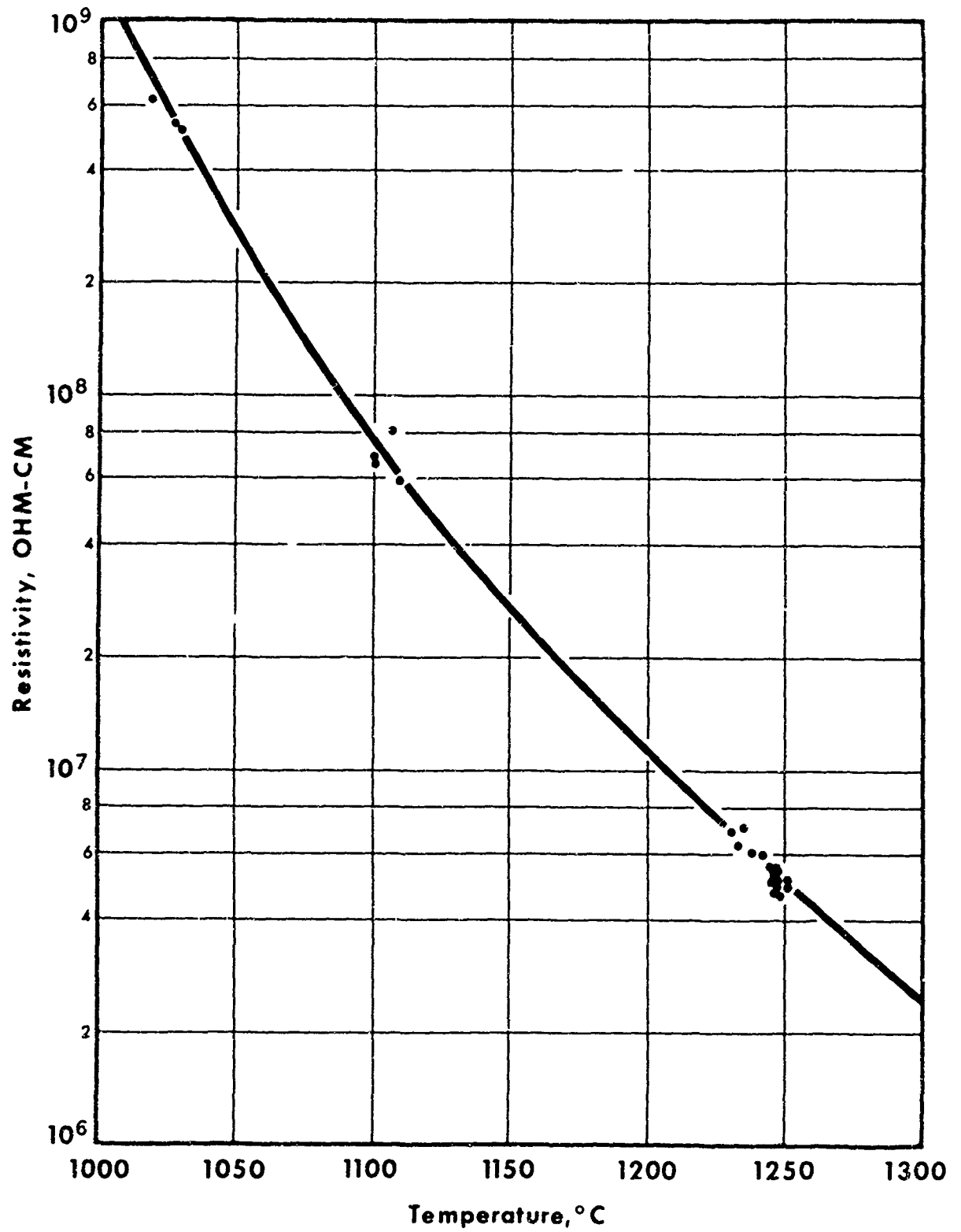
FIGURE II-6. TEMPERATURE DEPENDENCE OF RESISTIVITY FOR LUCALOX ALUMINA
