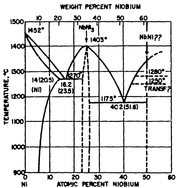
Figure III-19 Nickel-Niobium Phase Diagram 23
