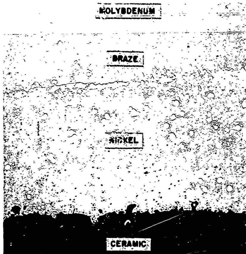
Alumina-to-Molybdenum Seal with Nickel Buffer Washers After 240 Hours at 1075°C (500X)
