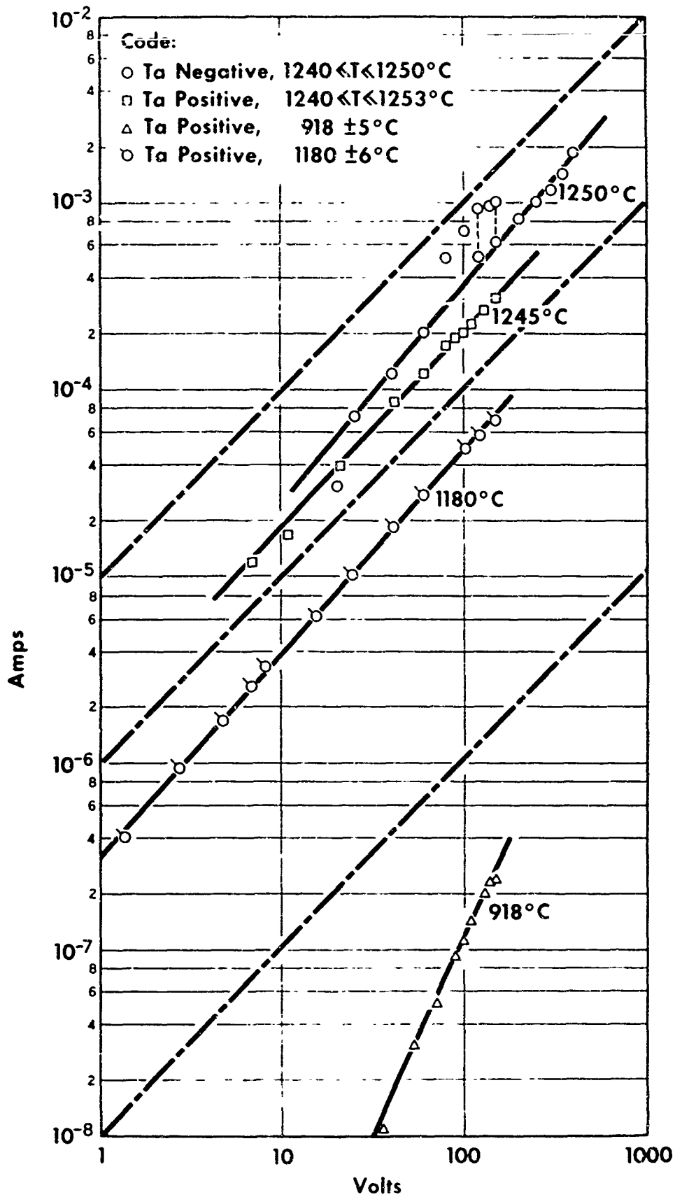
FIGURE II-5. CURRENT VERSUS VOLTAGE ACROSS INSULATOR
