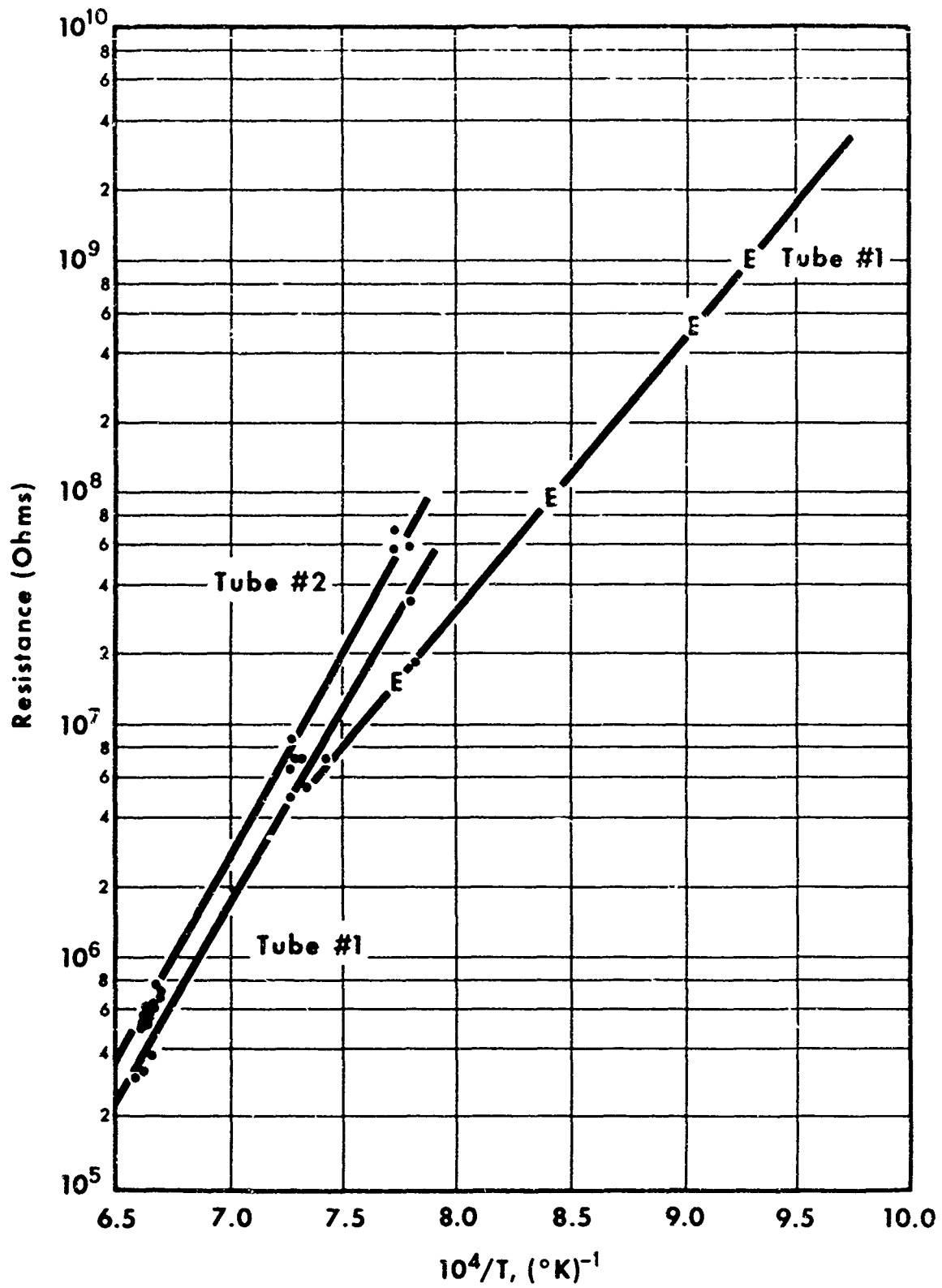
FIGURE II-4. TEMPERATURE DEPENDENCE OF RESISTANCE FOR TWO ALUMINA TUBES
