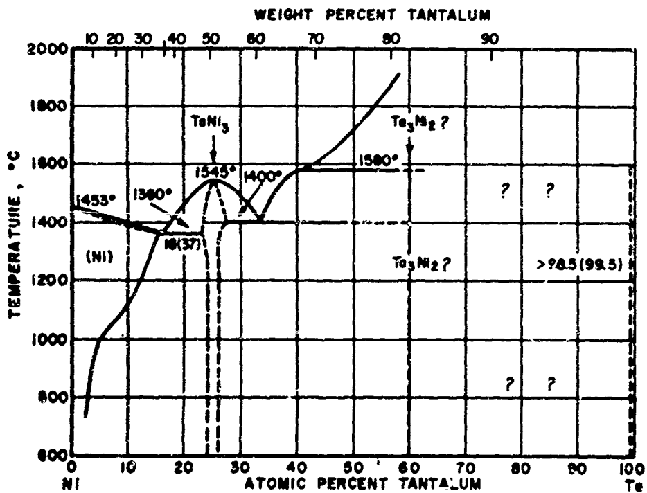
Figure III-20 Nickel-Tantalum Phase Diagram 24
