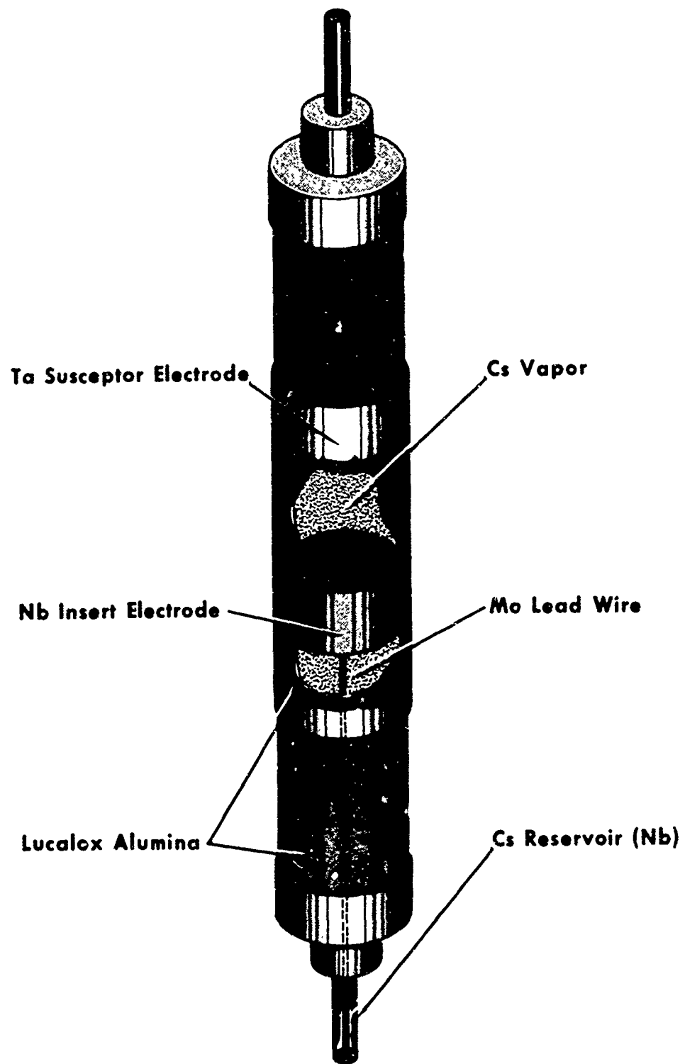
FIGURE II-1. LUCALOX ALUMINA CONFIGURATION FOR CONDUCTIVITY EXPERIMENT
