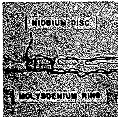
Before (250X) After 2 CNM brazed approx. 1300°C, 2 min., .0005-inch nickel shim
