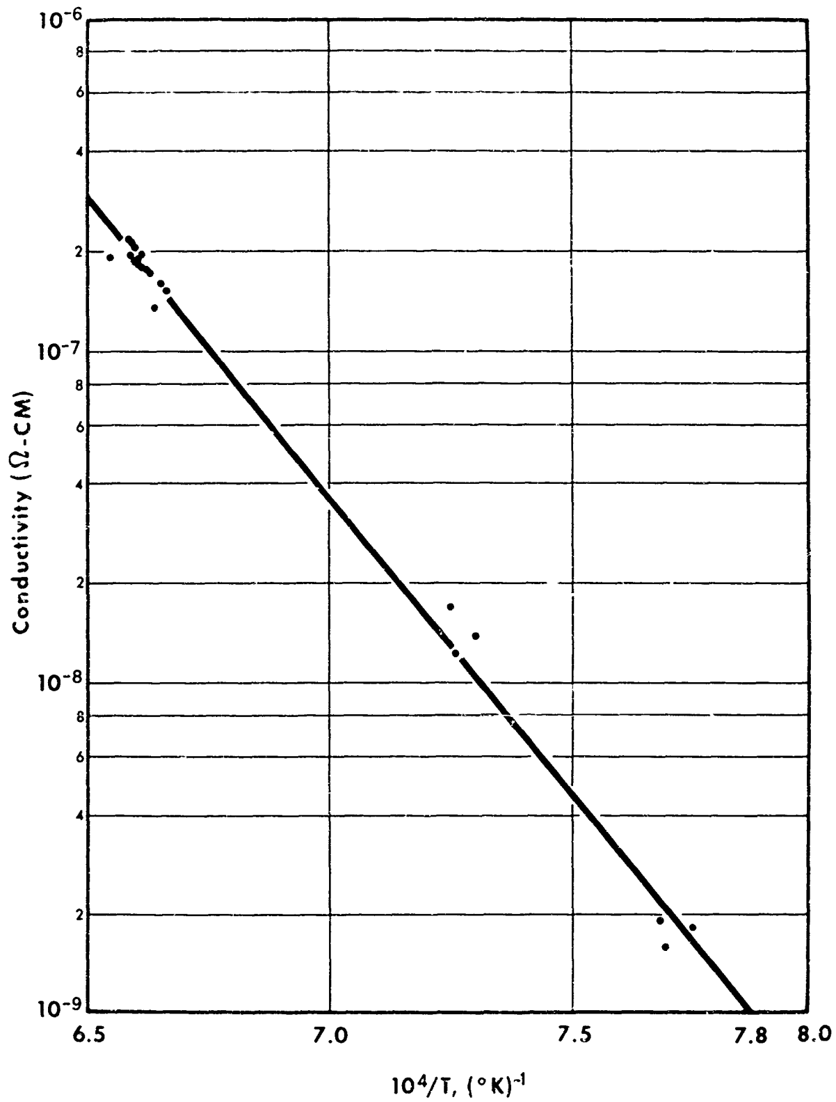
FIGURE II-7. TEMPERATURE DEPENDENCE OF ELECTRICAL CONDUCTIVITY FOR LUCALOX ALUMINA
