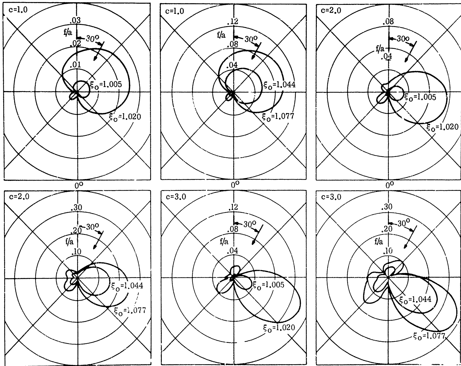
FIG. 6: SCATTERING PATTERNS IN PLANE OF INCIDENCE FOR HARD SPHEROIDS, PLANE WAVE INCIDENT 30^\circ OFF NOSE (Spence and Granger, 1951). f \equiv \lim_{r \rightarrow \infty} r e^{-ikr} \psi^s , \psi^s scattered field.
