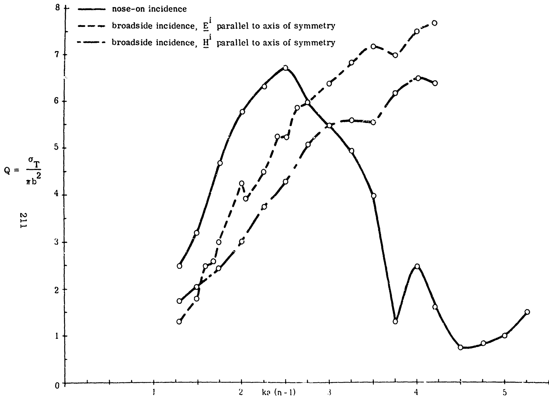
FIG 32; TOTAL CROSS SECTION OF A DIELECTRIC SPHEROID n = 1.26 , a/b = 2 (Greenberg et al. 1963b)
