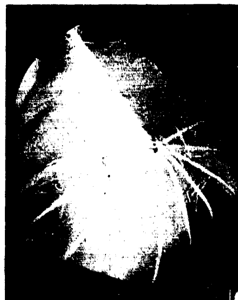
FIG 11. 32-IN. DIAMETER UNSYMETRICAL GLIDING PARACHUTE IN WIND TUNNEL (MODEL 1)
