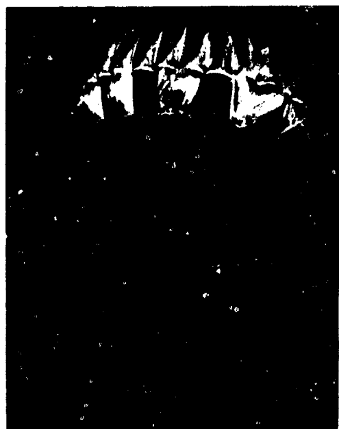
FIG 4. 26-IN. NOMINAL DIAMETER T-10 EXTENDED SKIRT PARACHUTE WITH UNSYMMETRICAL EXTENSIONS \alpha = 12^\circ \pm 3^\circ
