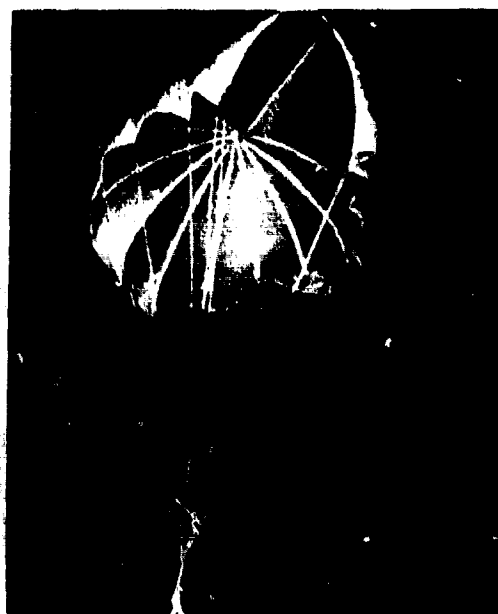
FIG 11. 32-IN. DIAMETER UNSYMETRICAL GLIDING PARACHUTE IN WIND TUNNEL (MODEL 1)
