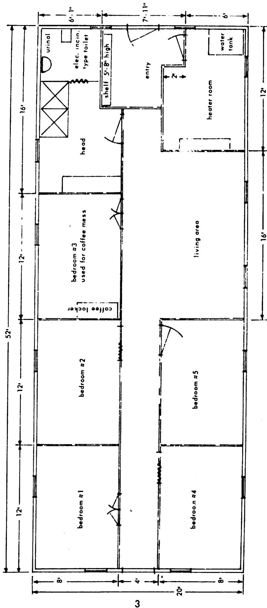
Figure 3. Floor plan of 20-foot by 52-foot T-5 quarters building.
