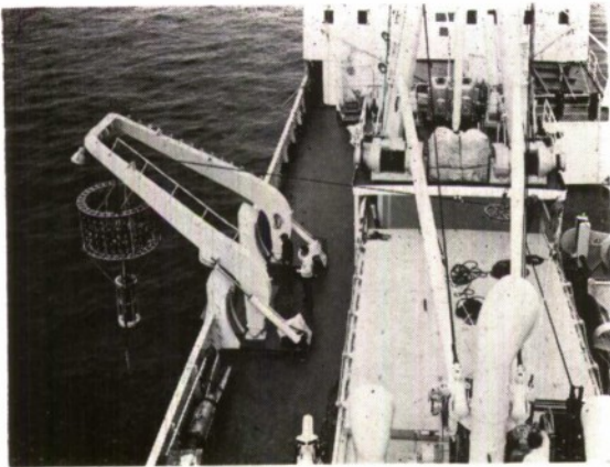
FIG. 2. Lowering an experimental deep sonar system from SACLANTCEN's research ship.
