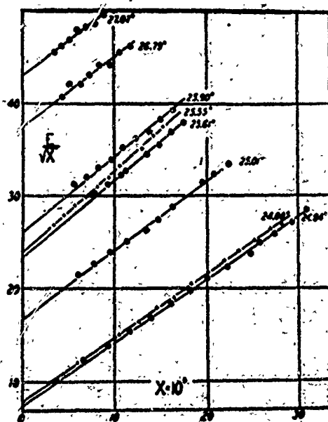
Verification of the law EX - \frac{1}{2} = M(t - t_0) + NX , whereby X = (m - m_0)/m_0
