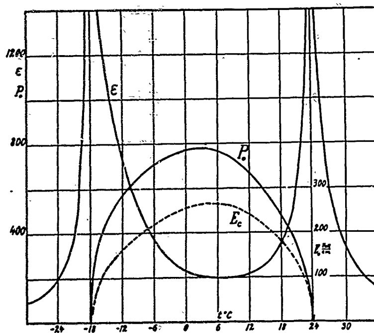
Permanent polarization P , coercive force E_c and dielectric constant for small fields of Rochelle salt in the ferroelectric temperature range.
