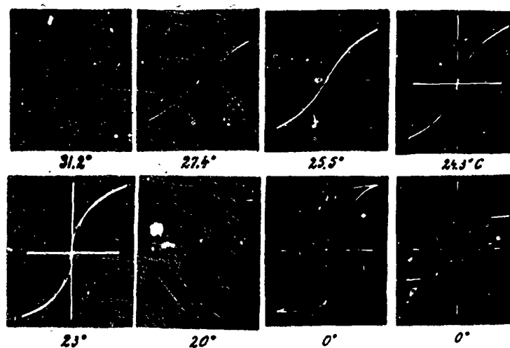
Polarization curves of Rochelle salt. Upper row: for temperatures above the upper Curie point, lower row: Hysteresis loops for temperatures between the Curie points.
