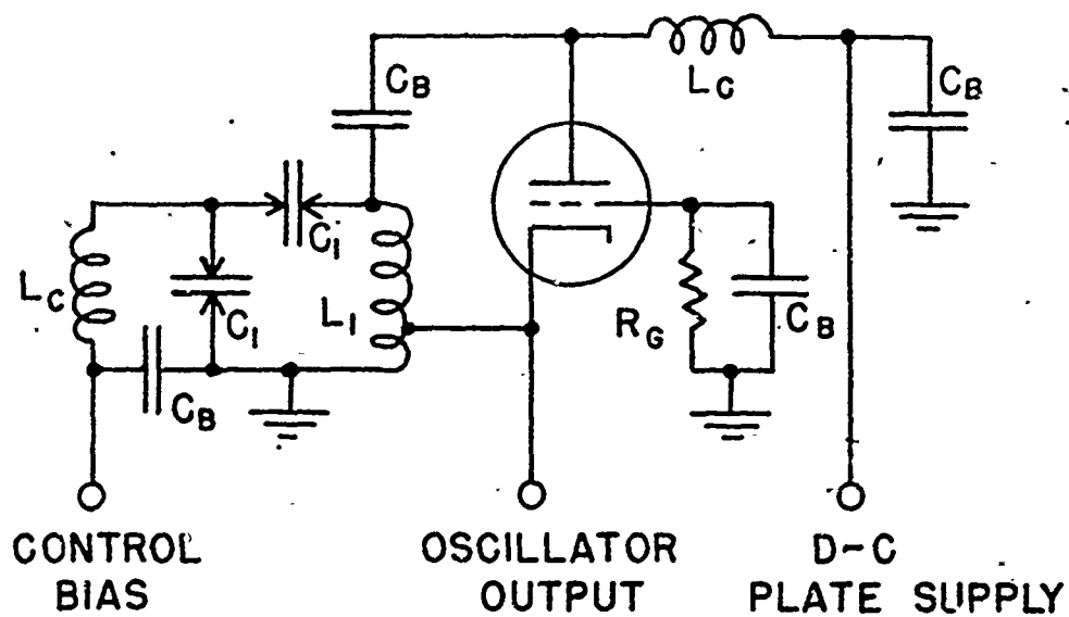
FIG. 38. FREQUENCY CONTROL BY NONLINEAR CONDENSERS.
