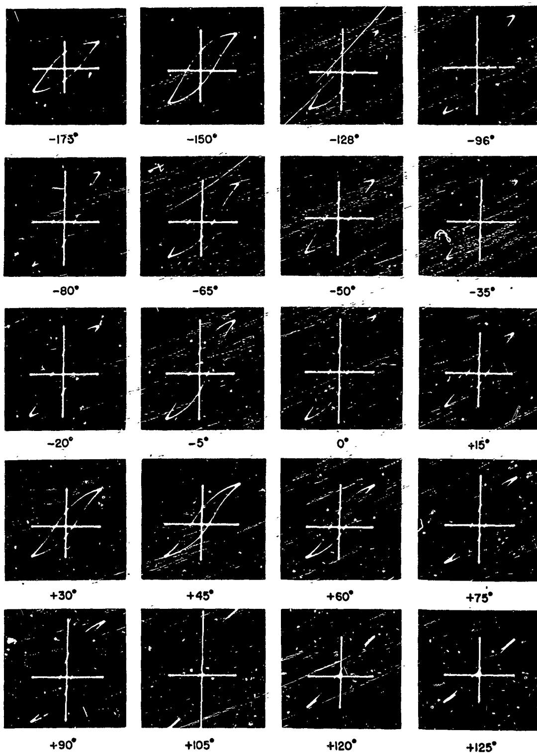
Fig. 4. Polarization Curves for \text{BaTiO}_3 (von Hippel 28 )
