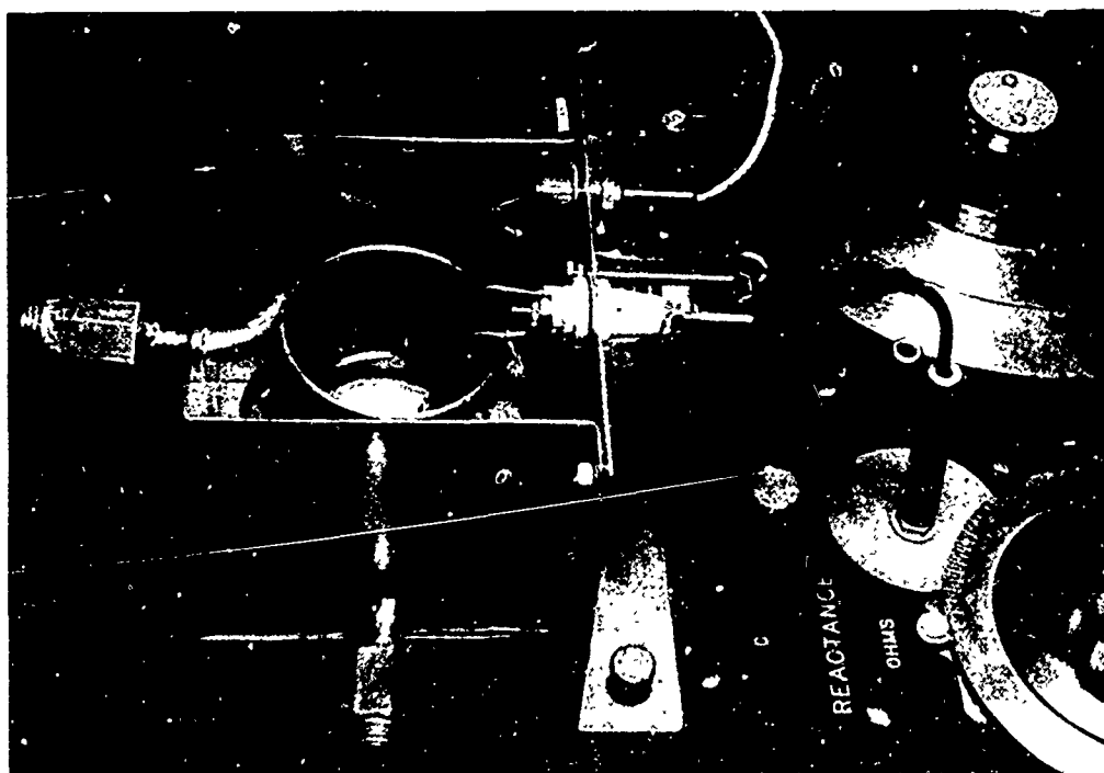
Fig. 6. Mounting arrangement showing connections to impedance bridge.
