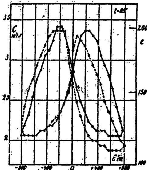
The reversible dielectric constant of Rochelle salt in the ferroelectric temperature range. The curve is the derivative of a hysteresis loop.
