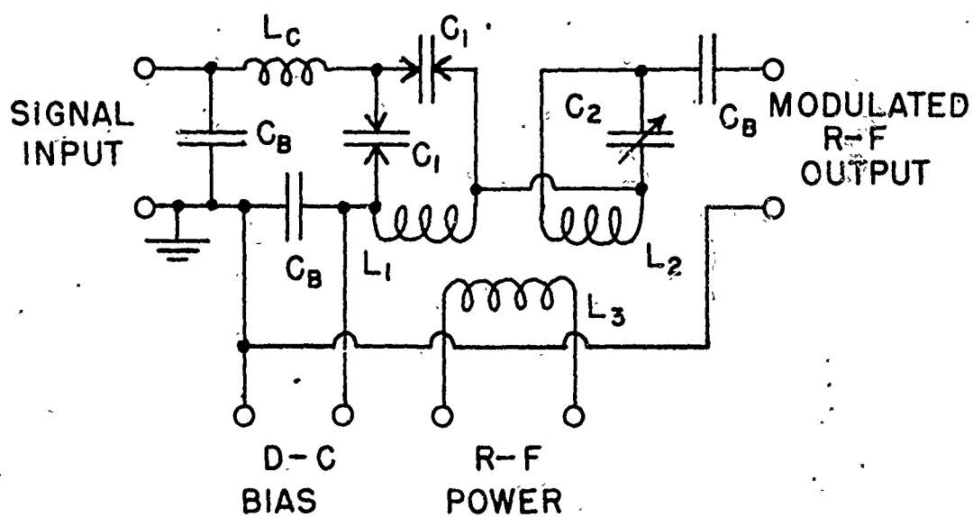
FIG. 40. AMPLITUDE MODULATOR CIRCUIT 40.
