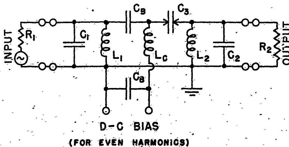
FIG. 39. NONLINEAR CONDENSER AS A HARMONIC GENERATOR.
