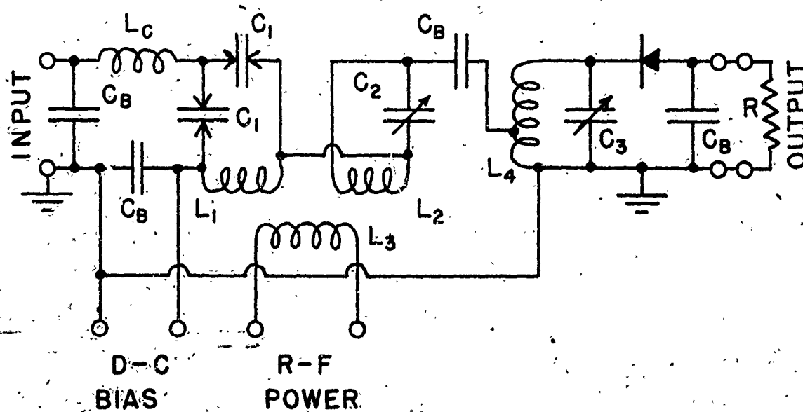
FIG. 41. DIELECTRIC AMPLIFIER 41.
