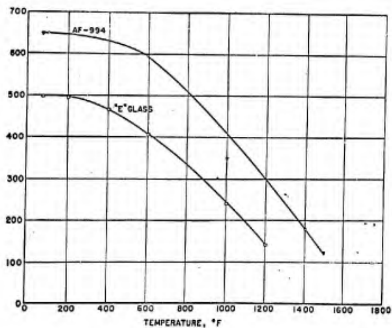
FIG. 9 - STRENGTH OF FIBERS AT ELEVATED TEMPERATURE (AF-994 AND "E" GLASS)
