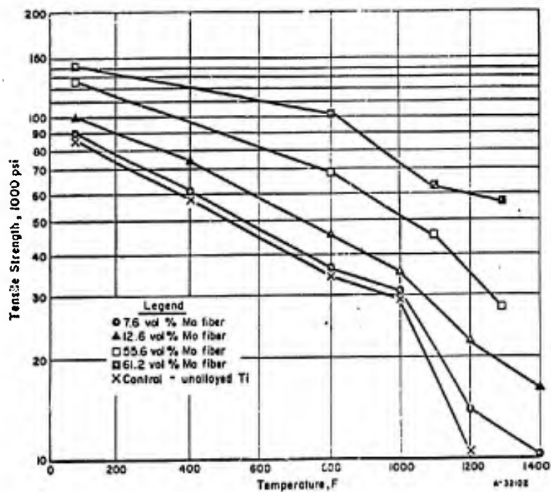
Figure 107. Tensile strength of staple molybdenum fibre reinforced unalloyed titanium 34 (Clevite Research Centre) DMIC report 117, 1959
