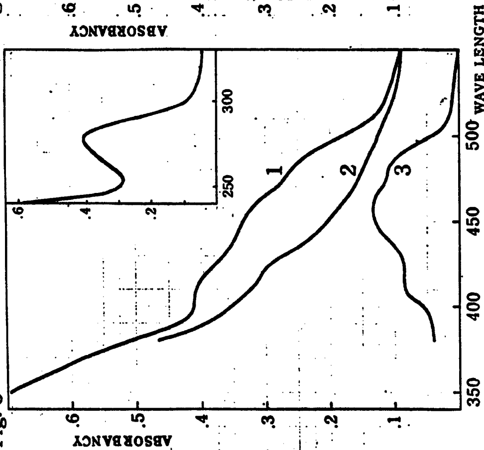
Absorption spectrum of PDC. 1 16.4 mg protein/2ml 1, oxidized form; 2, after addition of dithionite; 3, difference spectrum
