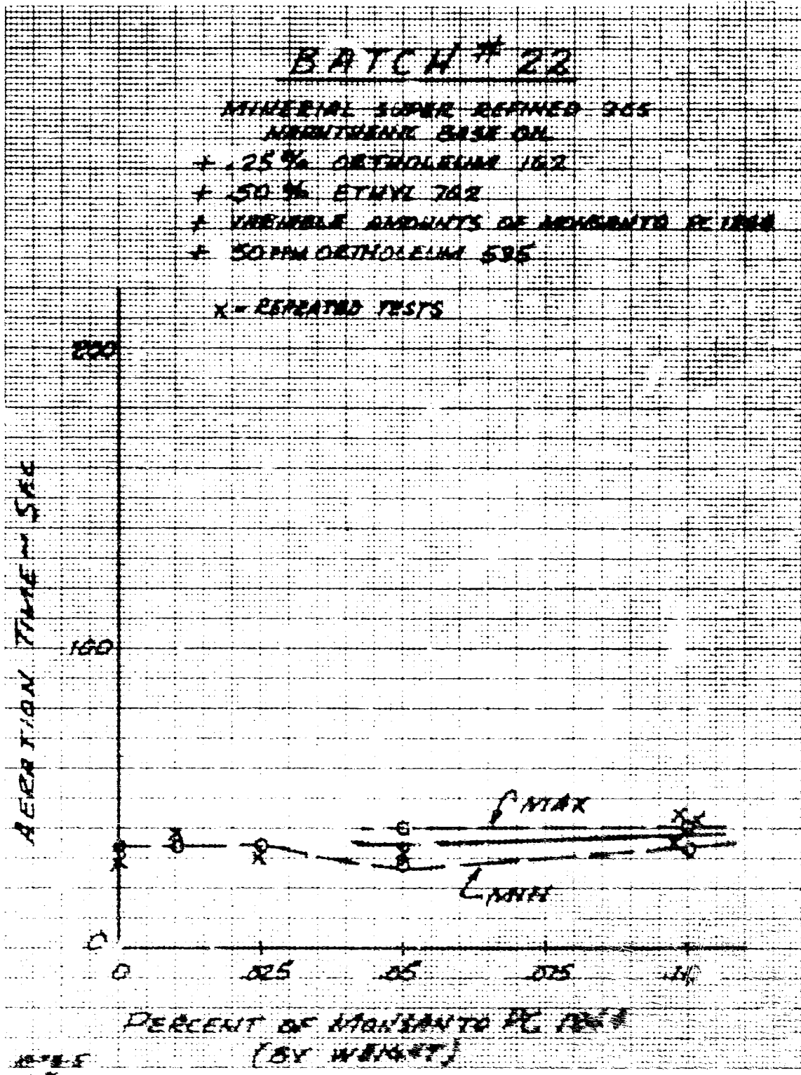
Aeration Time vs Percent of Nonsanto PC 104, Batch 22
