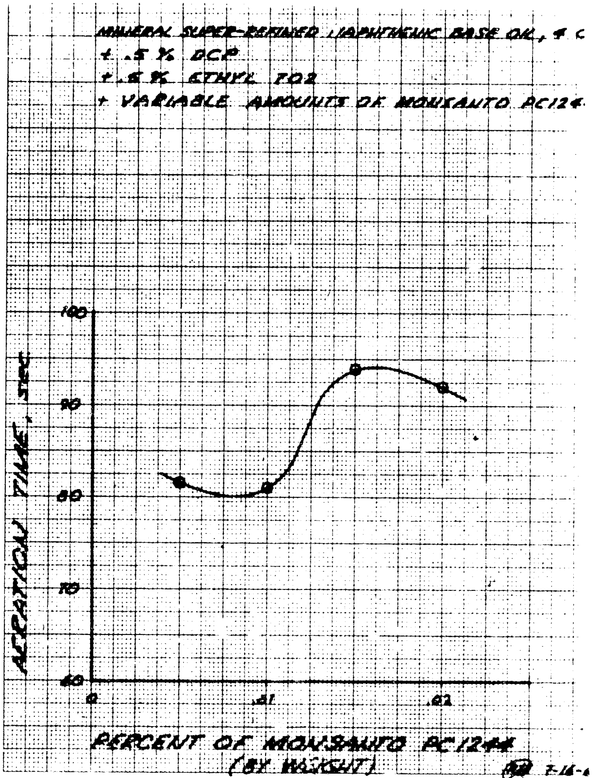
Aeration Time vs Percent of Monsanto PC-1244 (0.20% Ortholeum 162)
