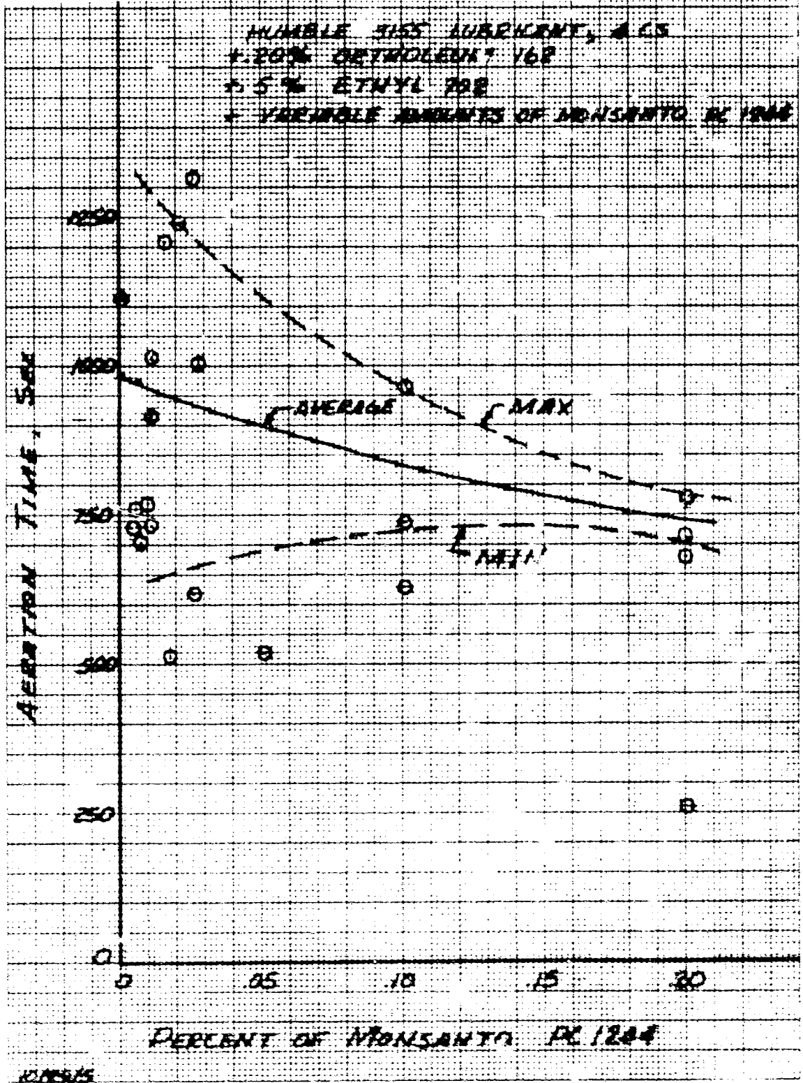
Aeration Time vs Percent of Monsanto PC-1244 (Didodecyl Phosphate Additive)
