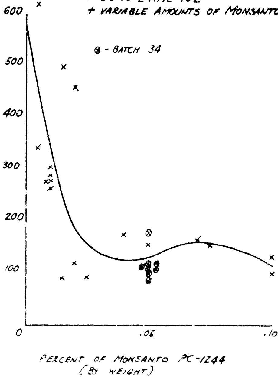
Aeration Time vs Percent of Monsanto PC-1244 (Dioctyl Phosphate Additive)
