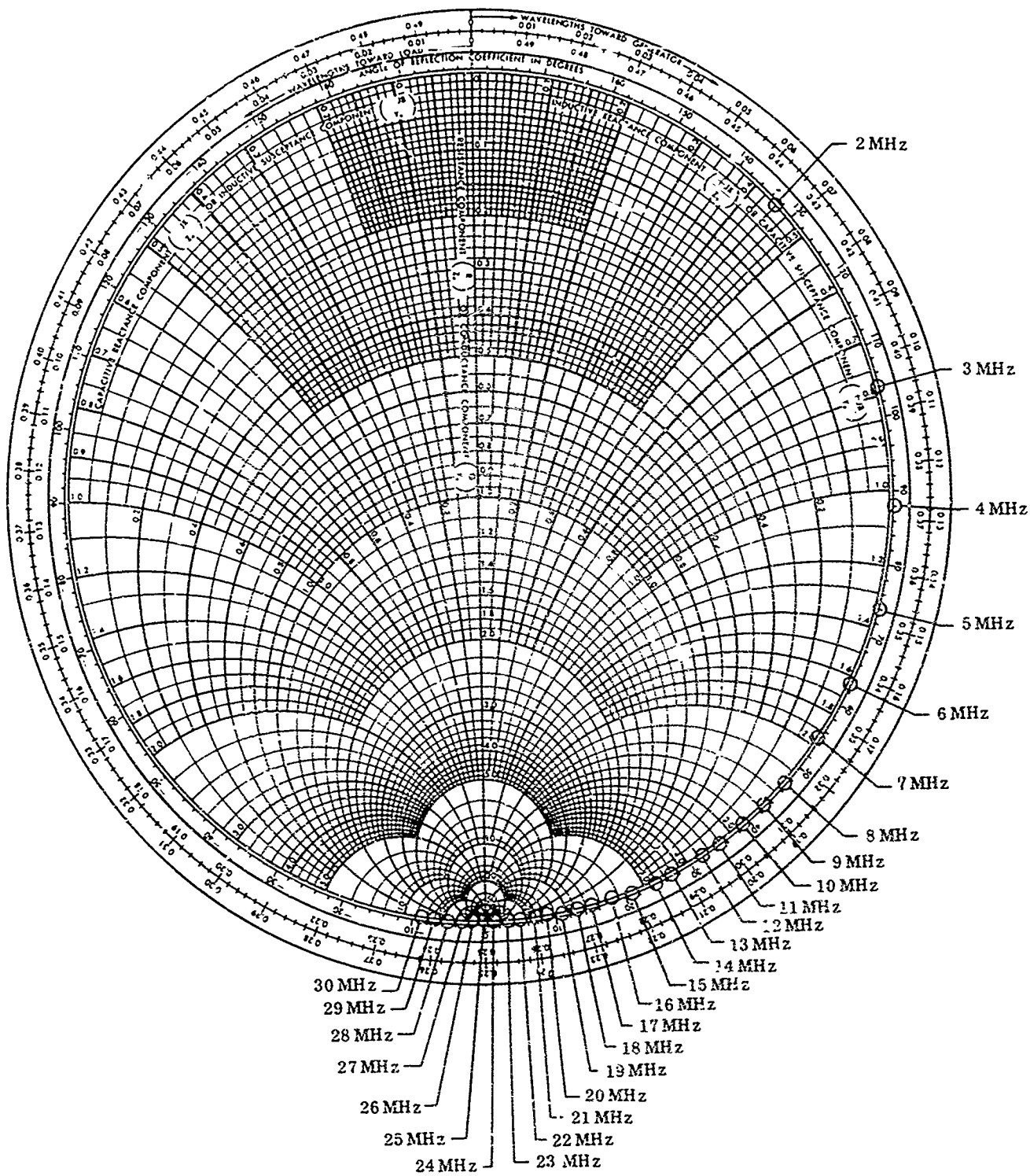
Fig. 4. Full-Scale 2-Turn Loop Impedance Characteristics
