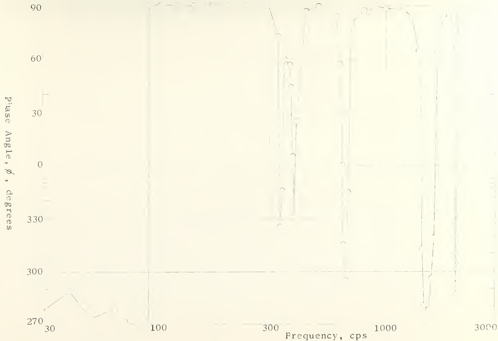
Fig. 12. Phase Angle \phi vs Frequency. Tip-driven Steel Cantilever Beam, 13 in x 2 in x 0.5 in. Direct Drive.
