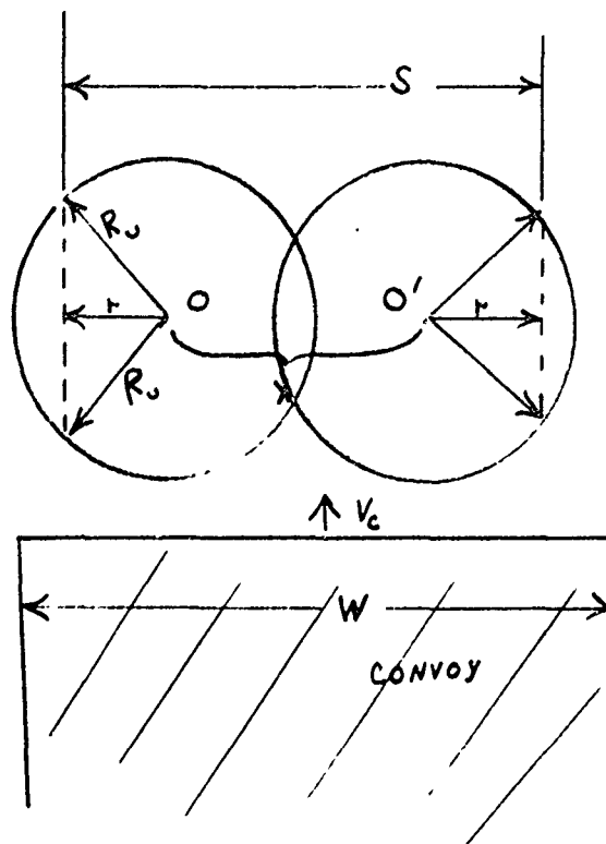
Diagram of Convoy Escort Search Pattern
