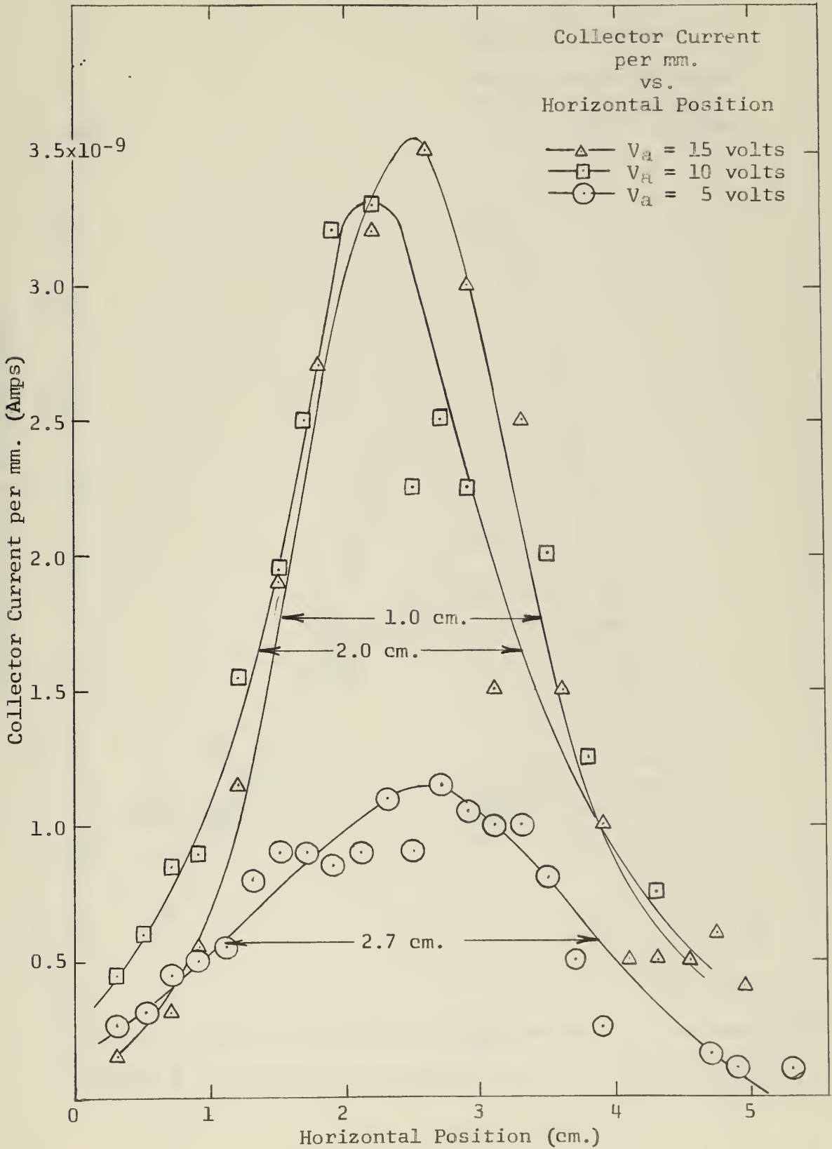
Figure 7. Horizontal Beam Profile at x = 6.7 cm.
