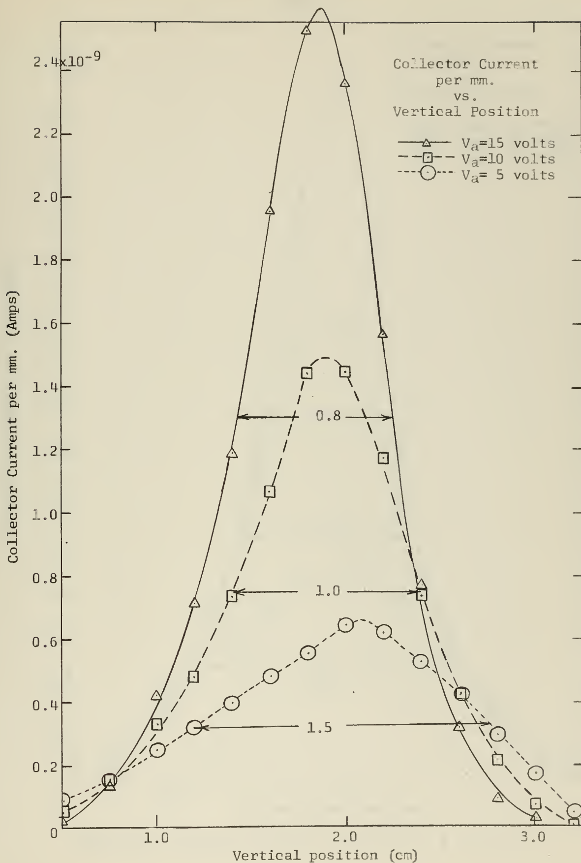
Figure 9. Vertical Profile, x = 5.1 cm, T = 825^\circ\text{C}
