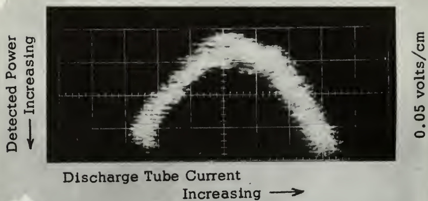
(a) Oscillogram of plasma resonance
