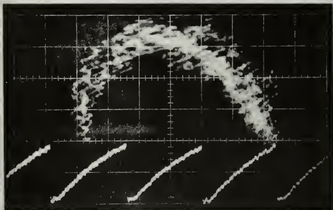
(b) Discharge Current = 240 ma f_0 = 480 \text{ mc/s}
