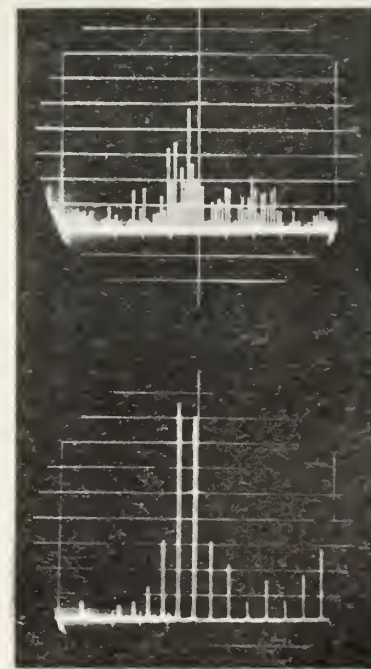
FIG. 5 . Center Freq. 60 Mc/s. Top photo -- Resistive leads with 0 db I.F. attenuation. Bottom photo -- One Mc/s markers.
