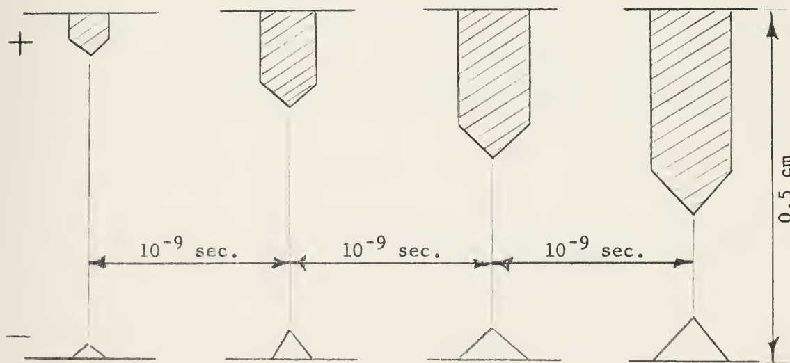
Fig. 2. Growth of a Spark in air across 0.5 cm gap with time intervals of 10^{-9} seconds
