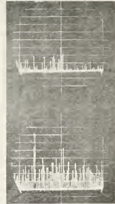
FIG. 17. Center Freq. 10 KMc/s. 1,5 Top photo -- Resistive leads with 0 db I.F. attenuation. Bottom photo -- Regular leads with 9 db I.F. attenuation.
