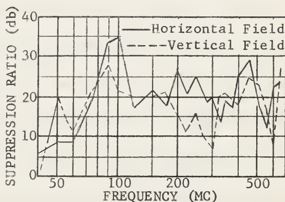
Suppression ratio given by resistive leads on 6-cylinder car.
