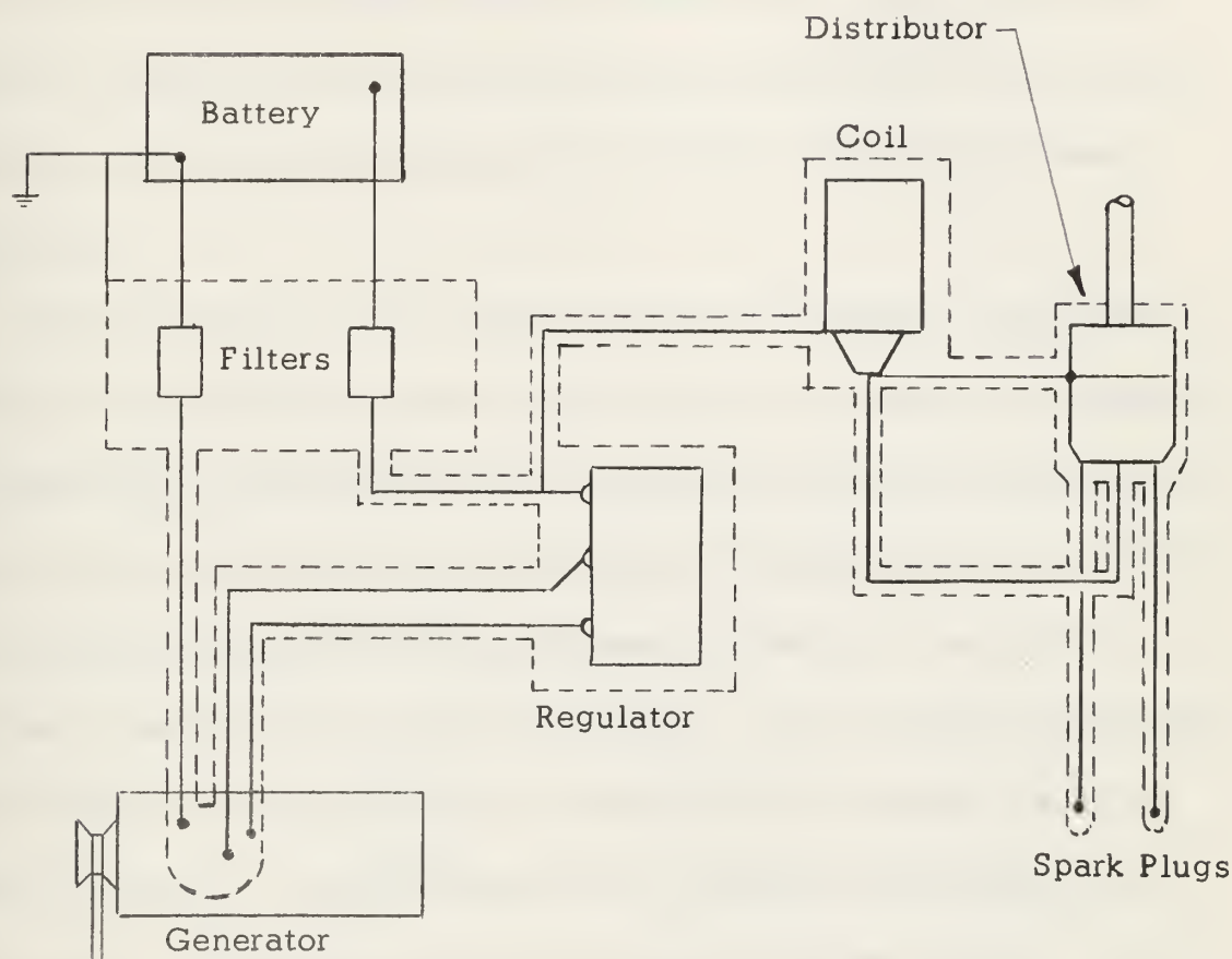
Fig. 1. Shielded Ignition System.
