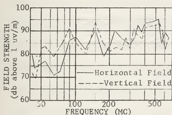
Field-strength of radiation from 6-cylinder cars at a distance of 30 feet.
