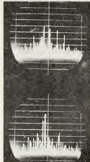
FIG. 8 . Center Freq. 200 Mc/s. 1 Top and bottom photos -- Regular leads with 8 db I.F. attenuation.
