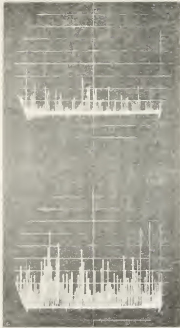
FIG. 15. Center Freq. 4 KMc/s. 1,3 Top photo -- Resistive leads with 0 db I.F. attenuation. Bottom photo -- Regular leads with 6 db I.F. attenuation.
