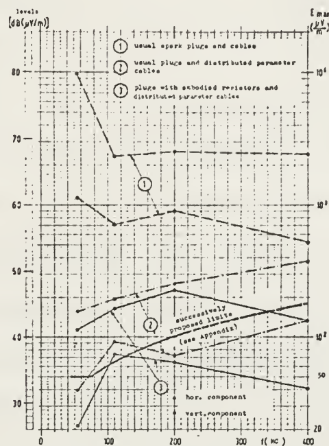
Fig. 7—Example of interference produced by a car without suppression and with two different means of suppression incorporated.
