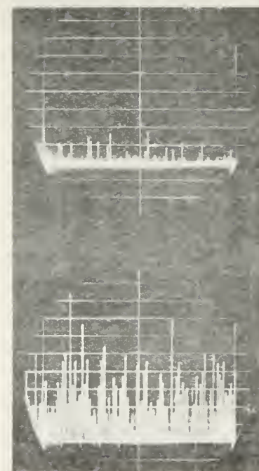
FIG.14 . Center Freq. 2 KMc/s. 1,2 Top photo -- Resistive leads with 0 db I.F. attenuation. Bottom photo -- Regular leads with 3 db I.F. attenuation.
