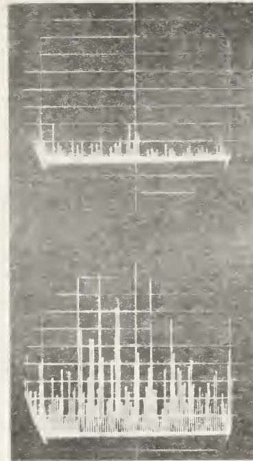
FIG. 16. Center Freq. 6 KMc/s. 1,4 Top photo -- Resistive leads with 0 db I.F. attenuation. Bottom photo -- Regular leads with 6 db I.F. attenuation.
