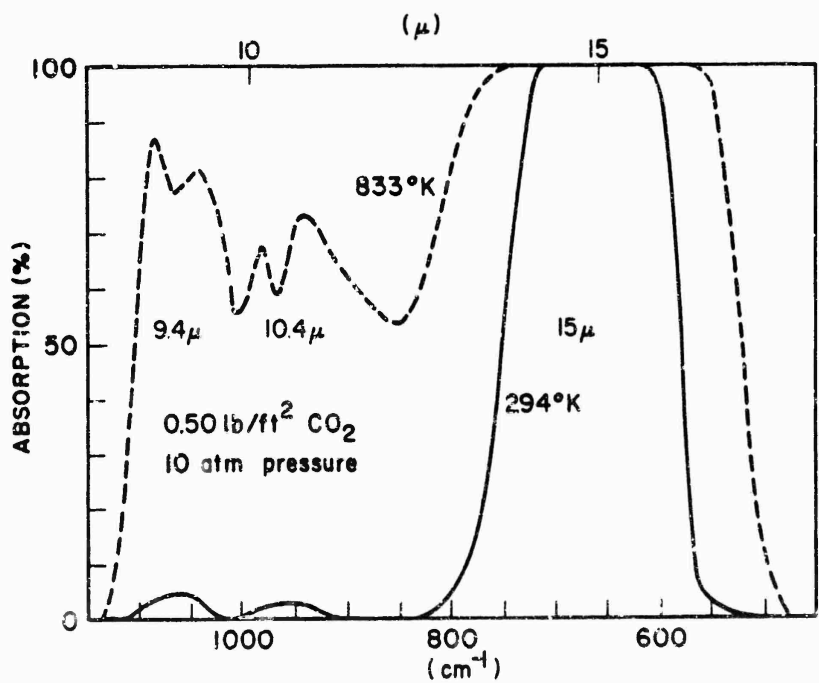
Fig. 2-11 Temperature Dependence of Carbon Dioxide 9.4-, 10.4-, and 15-Micron Bands. Data by Edwards (Ref. 7)
