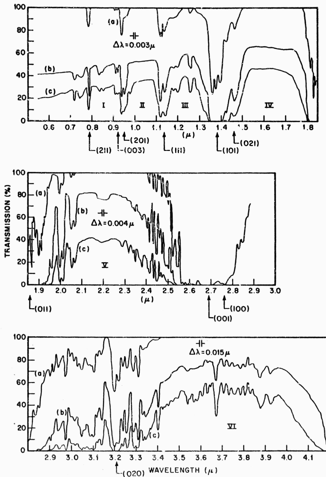
Fig. 3-5 Long-Path Atmospheric Transmission Curves, Showing Locations of Water Vapor Absorption Bands. Data by Taylor and Yates (Ref. 3)
