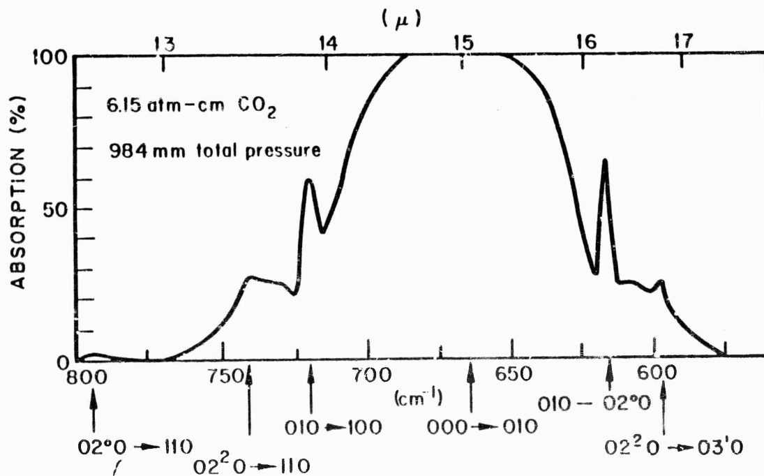
Fig. 2-7 Carbon Dioxide 15-Micron Band, Long Absorbing Path. Data by Burch et al. (Ref. 2)
