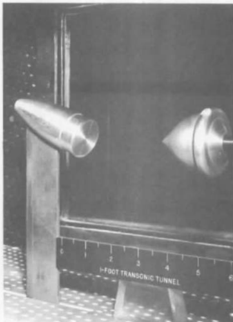
0.075-Scale Payload, x/D = 2, \alpha = 20 \text{ deg}
