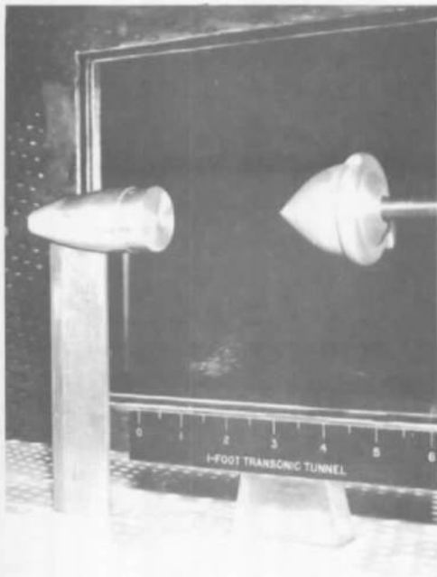
0.075-Scale Payload, x/D = 2, \alpha = 0 \text{ deg}
