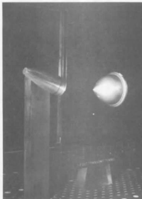
0.055-Scale Payload, x/D = 2, \alpha = 20 \text{ deg}
