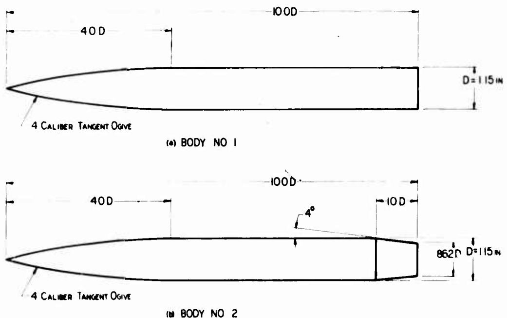
Figure 1. Body Configurations
