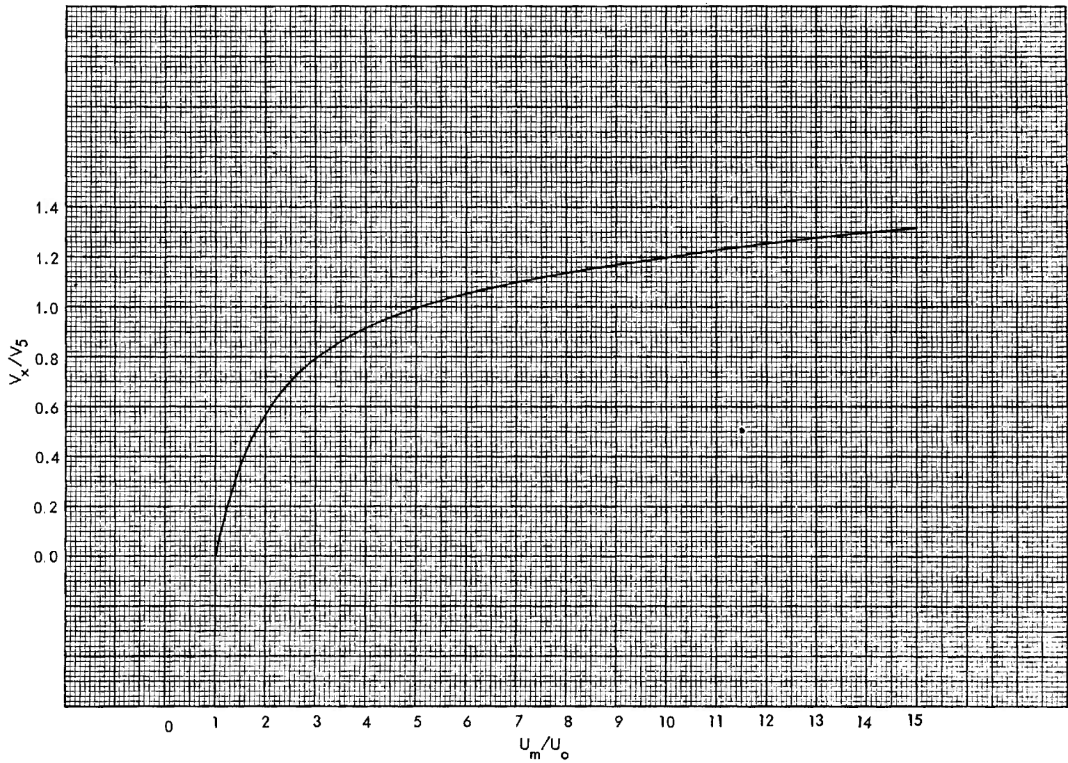
CHART 2-6. Relative Velocity Normalized to Unity at an Expansion Ratio of 5 as a Function of Expansion Ratio (Small Arms)
