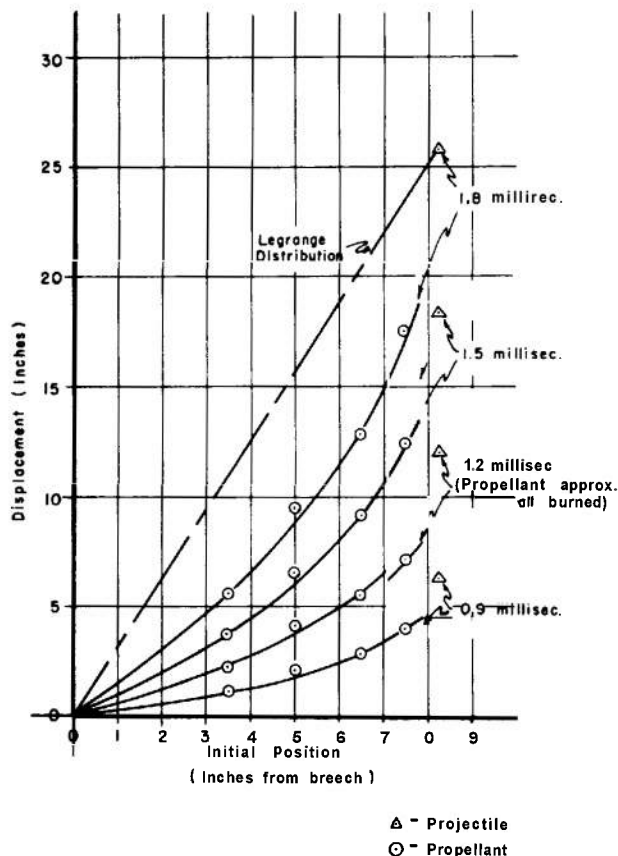
FIGURE 4-33. Distance Traveled by Radioactive Source as a Function of Initial Position Compared with the Displacement of the Gas Given by the Lagrange Approximation.
