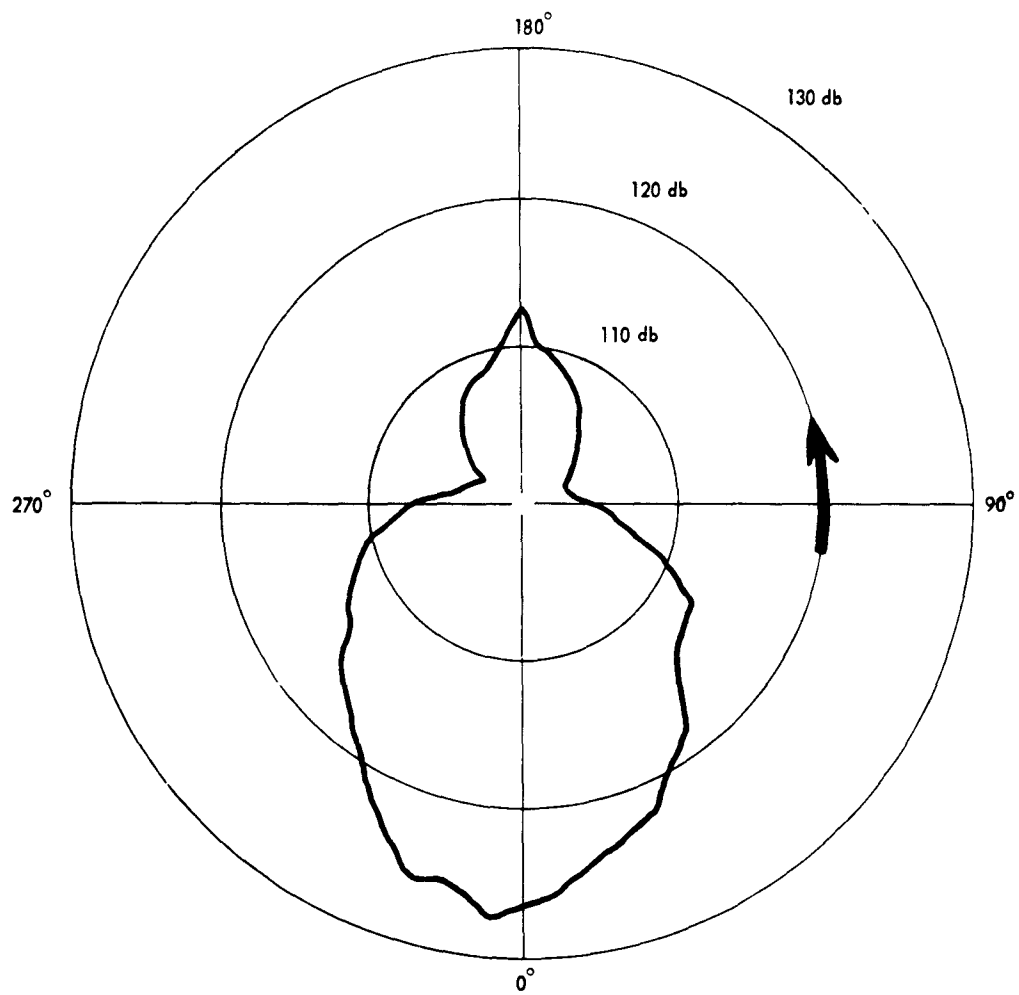
Fig. D1—Typical Directivity Pattern of Federal Siren Model 1000 TT 34
