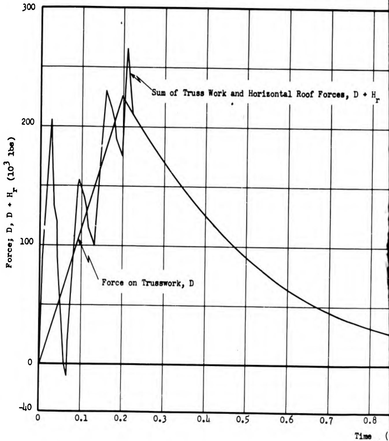
Fig. E.2.25 Force on Trusswork and Sum of Trusswork
