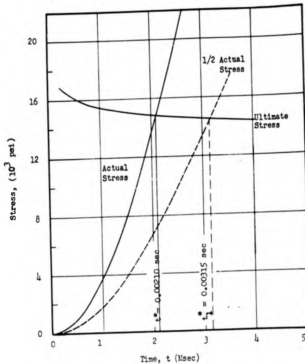
Fig. E.8.5 Actual Vs. Ultimate Stress ( t^* = time of break)
