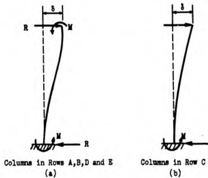
Fig. E.11.4 Column Deflection Curves of Building 3.3.4
