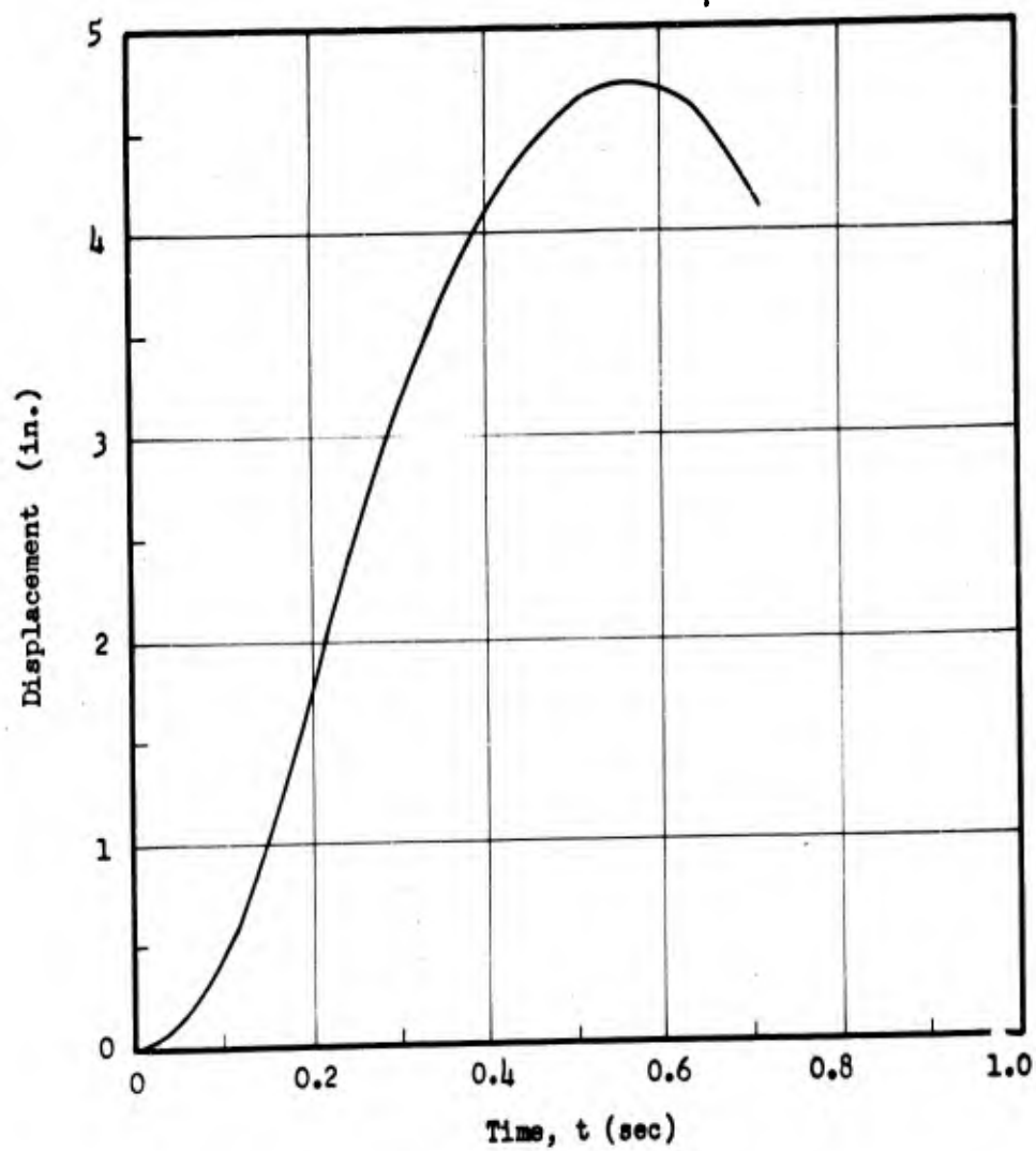
Fig. E.11.9 Displacement of Building 3.3.4
