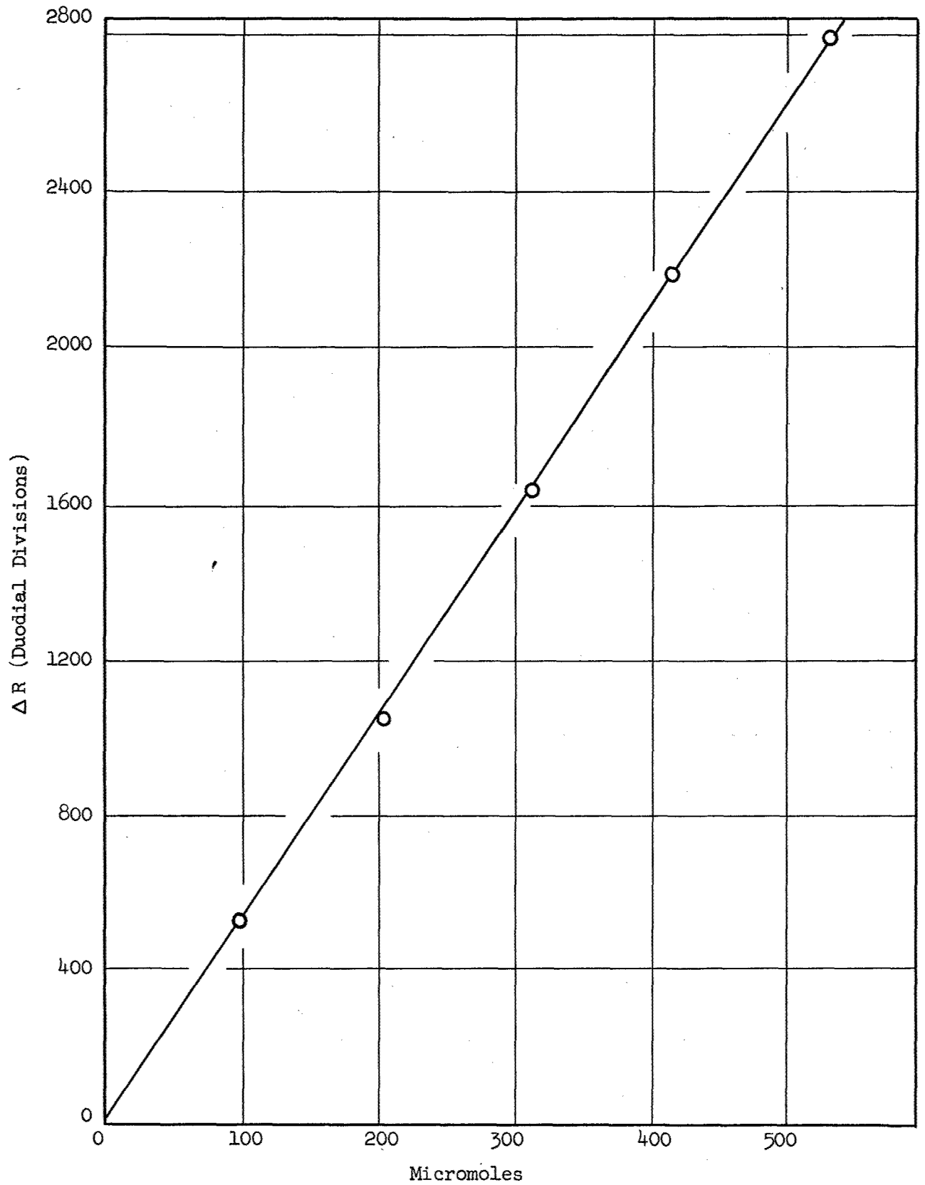
Figure 3. Ebulliometer Calibration
