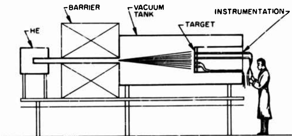
Fig. 3—HE plasma generator—Ablation experiment
