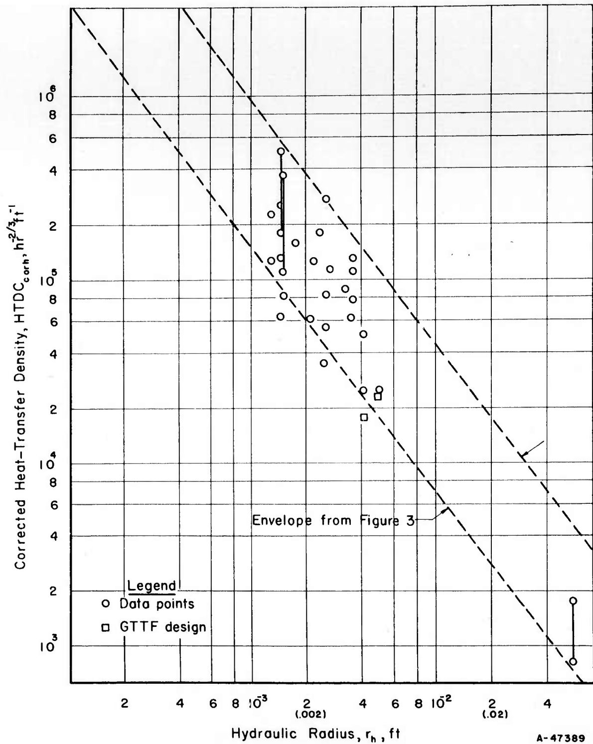
FIGURE 4. CORRECTED HEAT-TRANSFER DENSITY VERSUS HYDRAULIC RADIUS
