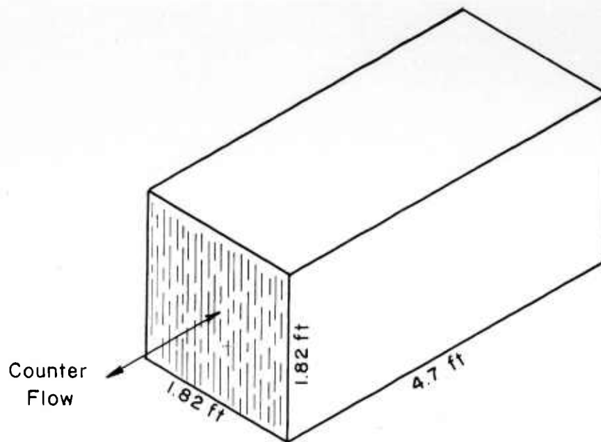
Recuperator 1
