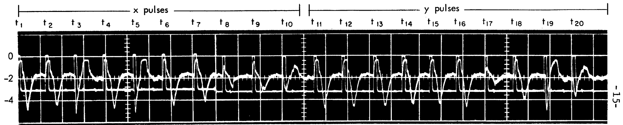
Fig. 8—Oscillogram of pen signal and strobe
