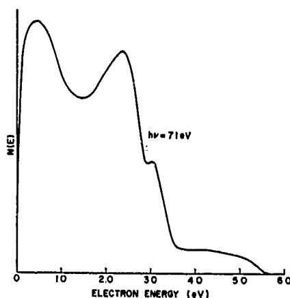
FIG. 36. ENERGY DISTRIBUTION OF PHOTOEMITTED ELECTRONS FROM COPPER-- h\nu = 7.1 ev.
