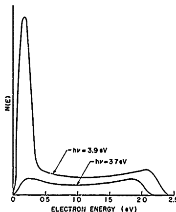
FIG. 23. ENERGY DISTRIBUTION OF PHOTOEMISSION ELECTRONS FROM COPPER-- h\nu = 3.7 ev, 3.9 ev.
