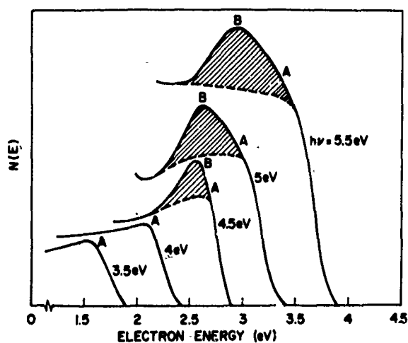
FIG. 27. EXPERIMENTAL EVIDENCE OF DIRECT AND INDIRECT TRANSITIONS IN COPPER.
