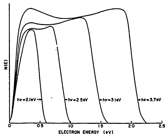
FIG. 21. ENERGY DISTRIBUTION OF PHOTOEMITTED ELECTRONS FROM COPPER-- h\nu \leq 3.7 eV.
