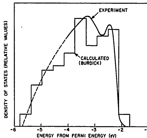
FIG. 34. DENSITY OF STATES OF d-BAND OF COPPER.
