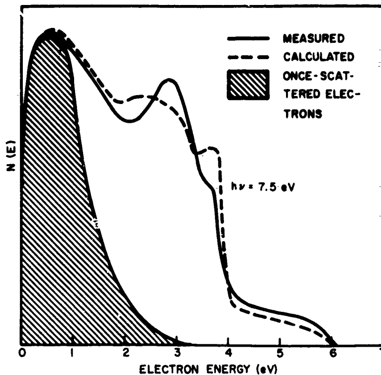
FIG. 41. CALCULATED AND MEASURED ENERGY DISTRIBUTION OF PHOTOEMISSION ELECTRONS-- \hbar\omega = 7.5 ev.
