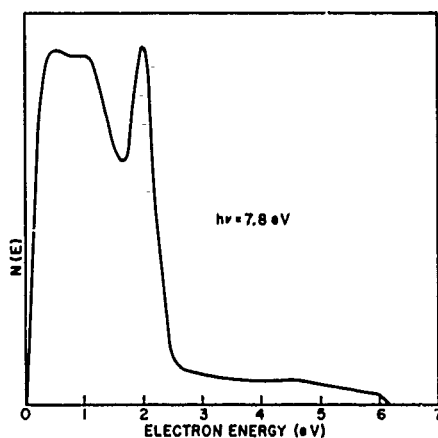
FIG. 58. ENERGY DISTRIBUTION OF PHOTOEMITTED ELECTRONS FROM SILVER-- h\nu = 7.8 eV.
