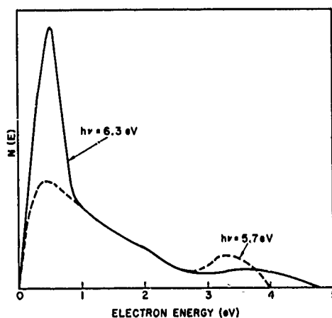
FIG. 57. ENERGY DISTRIBUTION OF PHOTOEMITTED ELECTRONS FROM SILVER-- h\nu = 5.7 eV, 6.3 eV.
