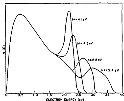
FIG. 54. ENERGY DISTRIBUTION OF PHOTOEMITTED ELECTRONS FROM SILVER-- K\omega = 4.1 ev to 5.4 ev.
