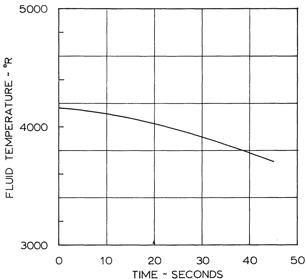
Fig. 26 Matrix Exit Air Temperature History
