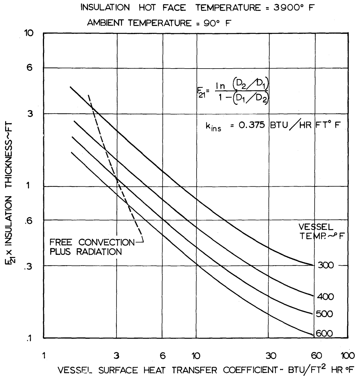
Fig. 2d Insulation Thickness
