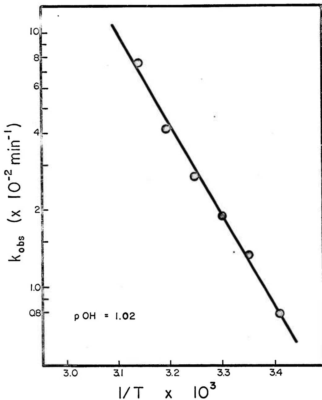
Fig. 11 Arrhenius type plot of logarithm of observed rate constant vs reciprocal absolute temperature for the hydrolysis of (III) at constant pOH = 1.02 .
