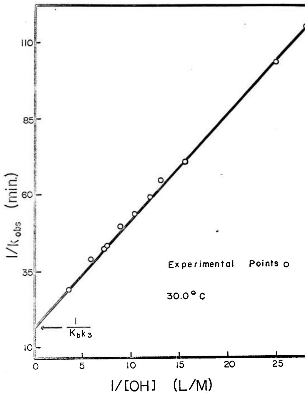
Fig. 7 Plot of reciprocal observed reaction rate vs reciprocal (\text{OH})^- concentration showing essentially linear relationship with intercept value of \frac{1}{K_b k_3} .
