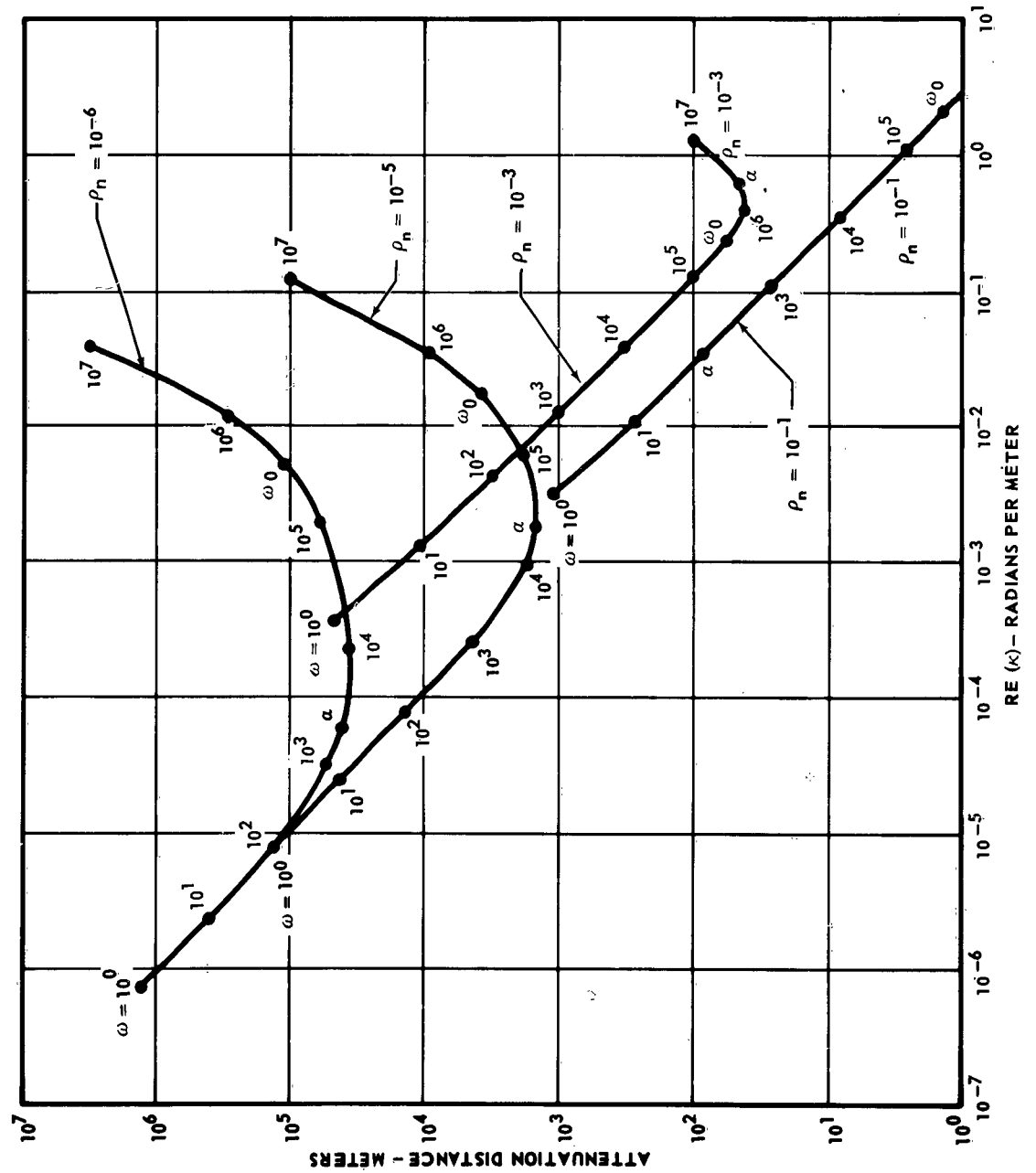
EFFECT OF NEUTRAL GAS DENSITY ON ATTENUATION DISTANCE
