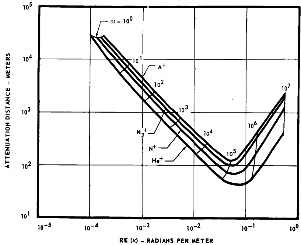
EFFECT OF MOLECULAR WEIGHT ON ATTENUATION DISTANCE
