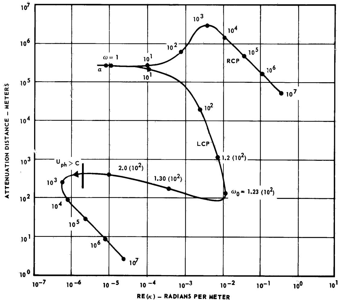
IONOSPHERIC PLASMA WAVE ATTENUATION vs WAVE NUMBER (300 KM ALTITUDE)
