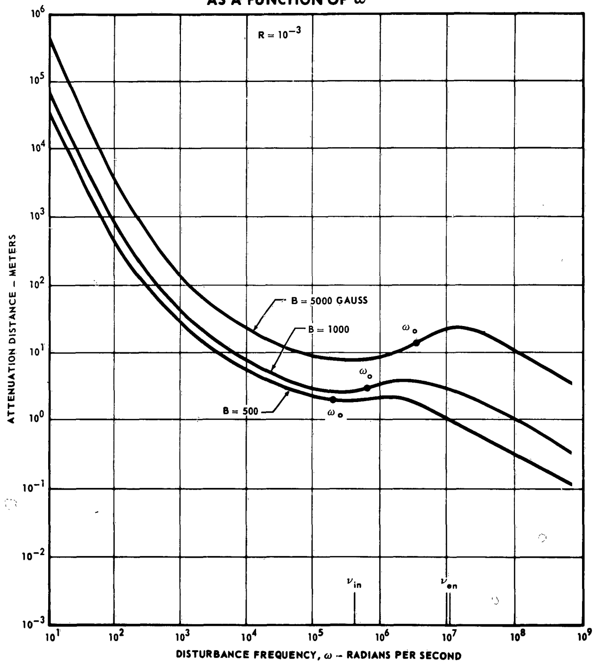
EFFECT OF MAGNETIC FIELD ON ATTENUATION DISTANCE AS A FUNCTION OF \omega
